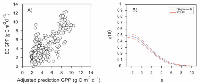
Figure 5. A) Adjusted predictions of GPP for the complete dataset from Bernal site using the leader model of the final ensemble of machine learning algorithms (EML) derived from Santa Rita site compared to estimates of GPP from EC data, r = 0.78 . B) Respective function of probability of agreement using a 1 \text{ g C m}^{-2} \text{ d}^{-1} as tolerable agreement between methods of estimation of GPP: EC data from the Bernal site and EML model for the Santa Rita site. The horizontal axis ( s ) represents the magnitude of the measurement, the vertical axis is the probability of agreement for the measurement, the red line is the confidence interval, p < 0.05 .
