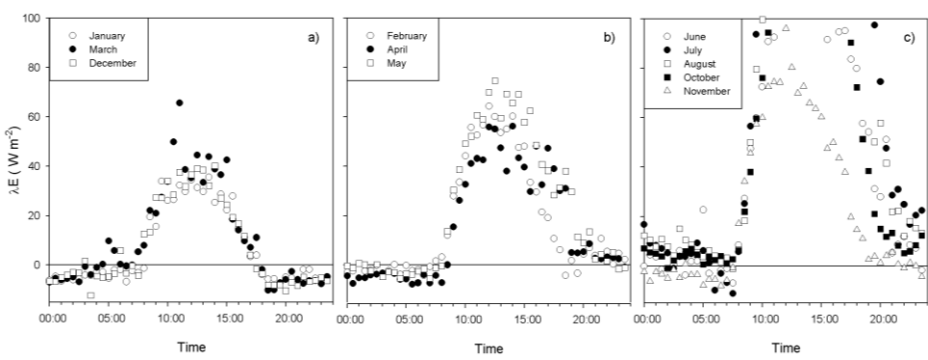
Figure 9. Latent heat flux daily trend at Bernal during different months emphasizing nighttime \lambda E . A) shows months with low rainfall in the previous month and predominantly negative \lambda E during nighttime (these months had low rainfall: 0.17, 11.3, 0.33 mm rainfall for January, March and December). B) shows months with low rainfall in the previous month and positive \lambda E after sunset (6.7, 7.3, 20.7 mm rainfall for February, April and May). C) shows months during the rainy season with \lambda E positive mainly due to soil wetness and antecedent rainfall of 43, 202, 9, 190, 34 mm for June, July, August, October and November. Plot C) is out of scale in the y axis for compatibility with the other plots.
