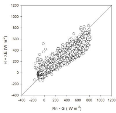
Figure 8. Closure of the surface energy balance from eddy covariance measurements averaged at 30 min between the turbulent fluxes ( H + \lambda E ) and available fluxes ( R_n - G ). Data is from march 30, 2017 to august 22, 2018 at Bernal site. The regression was y = 23.02 + 0.72 x , adjusted r^2 = 0.92 . Diagonal line represents the 1:1 relation.
