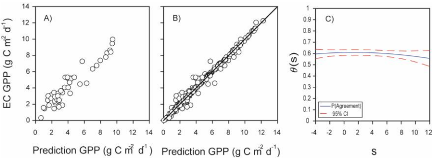
5 Figure 4. Agreement between predictions of GPP obtained with machine learning algorithms or derived from eddy covariance measurements at Bernal site. A) Example of one run predictions of GPP in the test dataset from Bernal site using the leader model of an ensemble of machine learning algorithms (EML), the test dataset was 15% of data, r=0.94 . B) Predictions for the complete dataset, r=0.99 , the diagonal line is the 1:1 agreement. C) Function of probability of agreement using a 1\text{ g C m}^{-2}\text{ d}^{-1} as tolerable agreement between methods of estimation of GPP corresponding to plot B). The horizontal axis ( s ) represents the magnitude of the 10 measurement, the vertical axis is the probability of agreement for the measurement, the red line is the confidence interval, p < 0.05.
