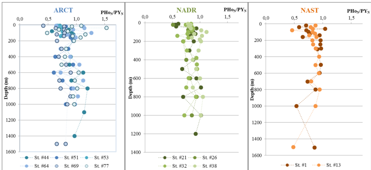
680 Figure 8: PAAS-normalized PHo/PY profiles by biogeochemical provinces.
