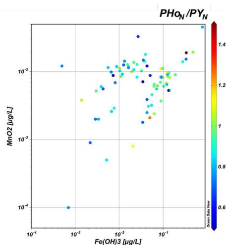
Figure 9: PAAS-normalized PHO N /PY N ratio as a function of Fe(OH) 3 and MnO 2 concentrations (in μg.L -1 ).
