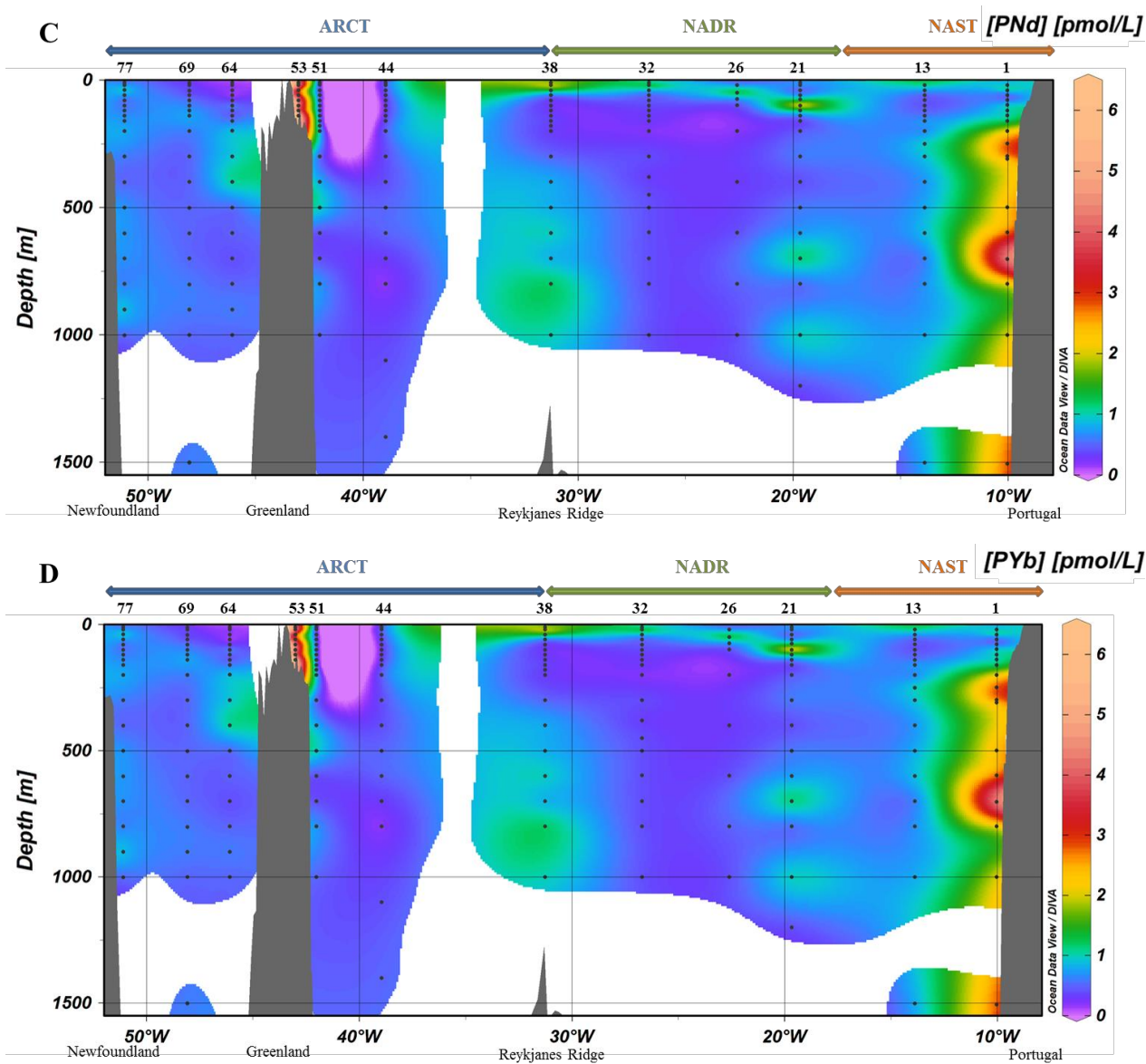
655 Figure 3: A. Profiles of particulate [Nd] and B. [Yb] concentrations superimposed on salinity (S) measured by CTD at every GEOVIDE station (Lherminier and Sarthou, 2017); in white, water masses characterized by OMP analysis (García-Ibáñez et al., 2018). At station #53, profiles are shifted to the bottom at a lower scale because of the shallow depth of the station. C. Particulate 660 [Nd] and D. [Yb] concentrations interpolated with the DIVA gridding function of Ocean Data View along the section defined in Fig. 1.
