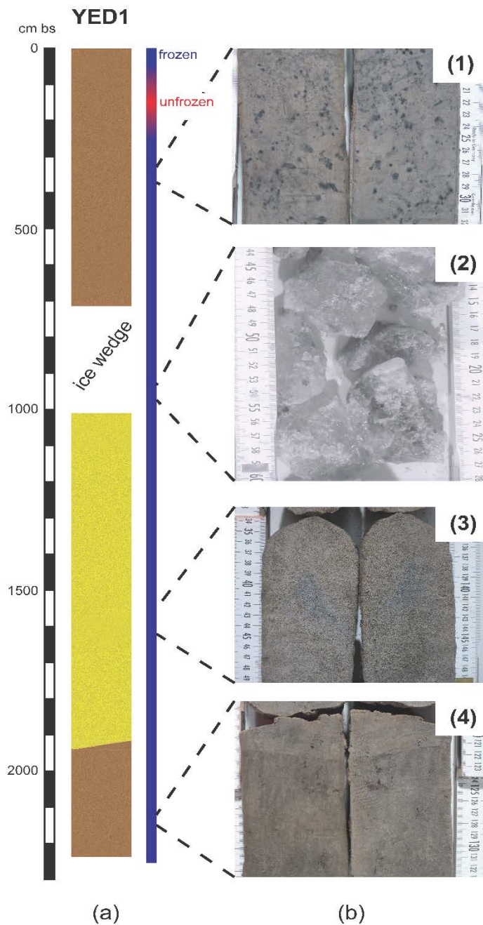
Figure 3 – a: overview of the Yedomoma core; depth given in cm bs; state after core retrieval is given by colors: blue = frozen, red = unfrozen; location of the ice wedge is labelled; brown illustrates silty sediments, yellow represents sandy sediments; b: detailed pictures of the YED1 core; (1) 332–317 cm bs, picture of unit Y1 showing black organic-rich inclusions within the grey silty matrix; (2) 960–944 cm bs, picture of the wedge ice in Y2; (3) 1549–1532 cm bs, picture of Y3, showing the coarse sandy material with no visible cryostructures or organic material; (4) 2133–2117 cm bs, picture of Y4, showing the grey silty matrix with some dark organic dots.
