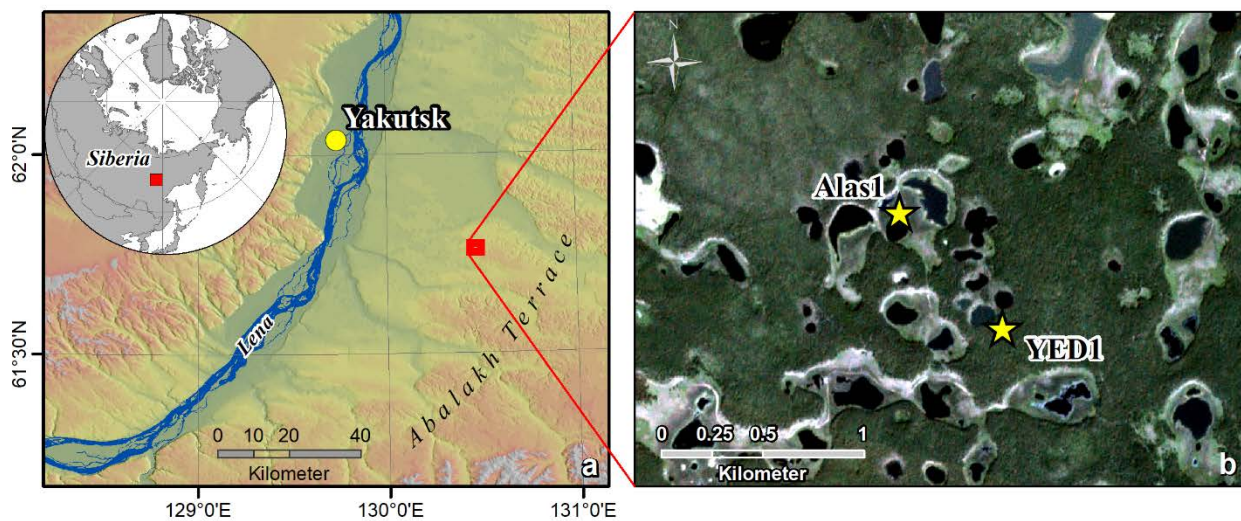
Figure 1 – Study site overview; a: location of the Yukechi Alas study site in Central Yakutia on the edge of the Abalakh Terrace (Circumpolar digital elevation model, Santoro and Strozzi, 2012); b: locations of the Alas1 and the YED1 coring sites within the Yukechi Alas landscape (Planet OrthoTile, acquisition date: 7 July 2018; Planet Team (2017)).
