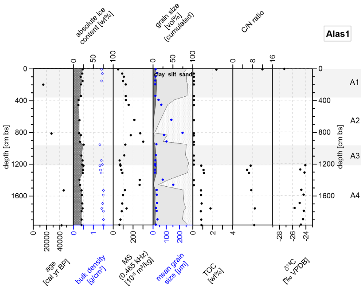
Figure 6 – Characteristics of the Alas1 core: radiocarbon age, absolute ice content, bulk density, magnetic susceptibility (MS), grain size composition, mean grain size, total organic carbon (TOC) content, carbon-nitrogen (C/N) ratio and stable carbon isotope ( \delta^{13}\text{C} ) ratio; grey/white areas mark different stratigraphic units (A1 to A4).
