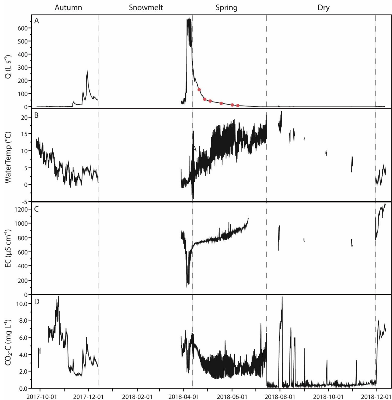
500 Figure 3. Time series of A) stream discharge (Q) with sampling days for \delta^{13}C -DIC highlighted by red dots, B) stream water temperature, C) electrical conductivity (EC), and D) CO_2 concentration for the study period September 26, 2017-December 12, 2018, with break for the ice- and snow-covered period December-March. The CO_2 data include periods when the sensor was above the water surface during dry periods in summer/autumn of 2018.
