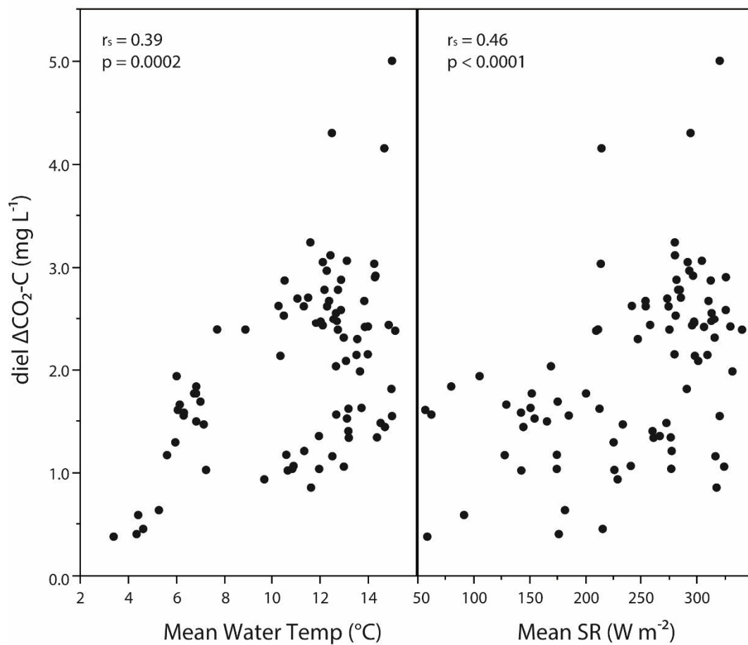
Figure 7. Diel amplitude in stream \text{CO}_2 concentration in relation to A) daily mean stream water temperature, and B) daily mean shortwave radiation (SR), covering the period April-July 2018. Statistics are given according to Spearman's rank correlation.
