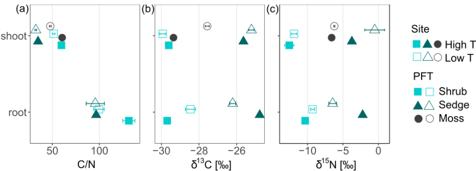
Figure 1: Carbon to nitrogen (C/N) ratios, \delta^{15}\text{N} [‰] and \delta^{13}\text{C} [‰] of shoot and root tissues from three plant functional types (PFTs; i.e. mosses, shrubs and sedges) and from two peatlands differing in temperature (high and low temperature indicated by High T and Low T, respectively). Symbols for shoots represent mean values with standard error ( n = 5 ), whereas symbols for roots give means of two or a single value (High T sedge root).
