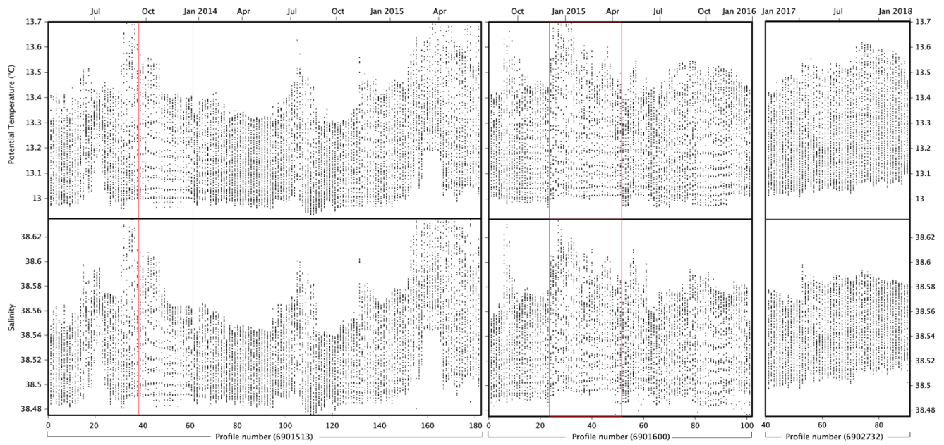
Figure 8: Temperature (upper panels) and salinity (lower panels) recorded in the range 300-1000 dbar with a vertical resolution of 10 dbar, by the three floats 6901513 (left panels), 6901600 (middle panels) and 6902732 (right panels) deployed in the Algerian Basin. In x-axis, number of the successive profiles with a resolution of one to seven days. The timeframe (in trimesters) is superimposed on top x-axis. The two episodes detailed in Section 3.2 are delimited by red lines.
