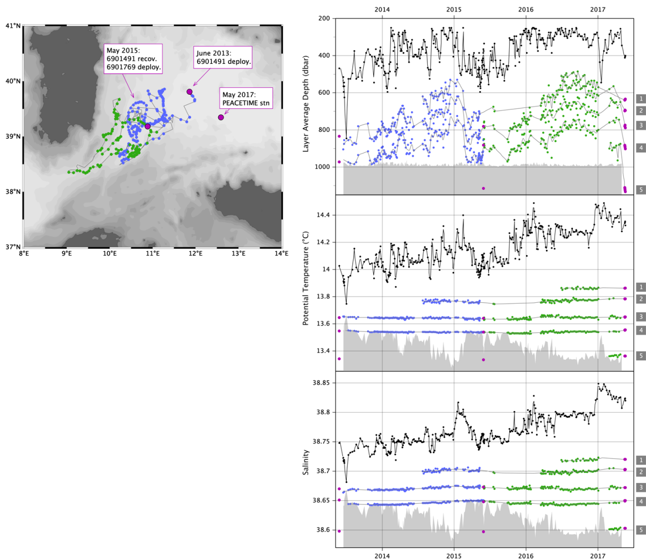
Figure 5: Left panel, location of staircase-detections along the trajectory of the consecutive floats deployed in June 2013 and May 2015. Right panels, time series of layer properties and depth (colored dots) of shipboard and float profiles with staircase detection. LIW properties and depth are indicated in black lines. The 1000 dbar limit is indicated in grey shadows. The layer numbering of the station PEACETIME (Table 3) is indicated inside grey boxes. All panels: station locations and layer properties are indicated in purple for shipboard profiles, in blue for the float 6901491 and in green for the float 6901769.
