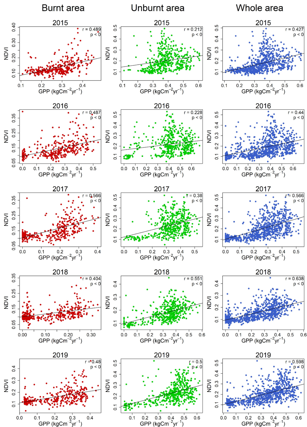
Figure S1. Correlation between modelled GPP output and Landsat-derived NDVI
