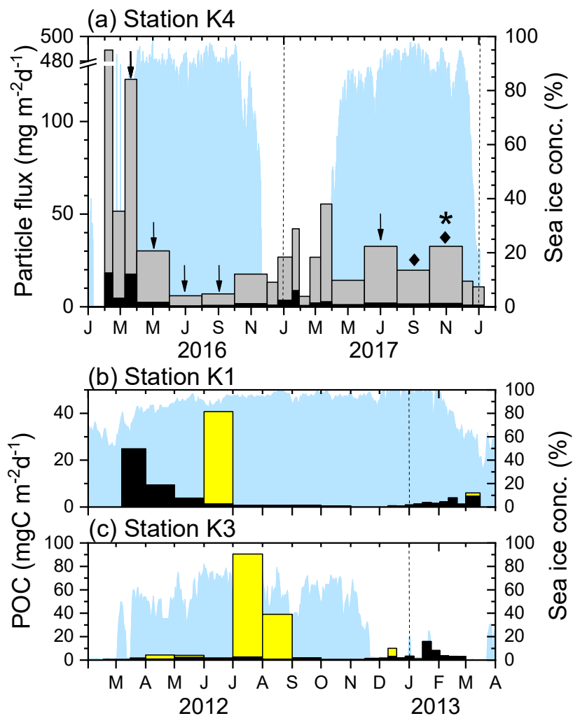
Figure 2: (a) Fluxes of sinking particles (gray bars) and POC (black bars) at Station K4. The tick marks on the x-axis indicate the start of each month. The arrows, diamonds, and the star respectively indicate the periods when worms, scallops, and the sea urchin were collected. (b) POC fluxes by worms (yellow bars) and sinking particles (black bars) at Stations K1 and (c) K3. Note that the y-axis scales differ. The dotted vertical lines denote the beginning of each year. The blue shading indicates the sea ice concentration. POC flux and sea ice data for Stations K1 and K3 were redrawn from Kim et al. (2019).
