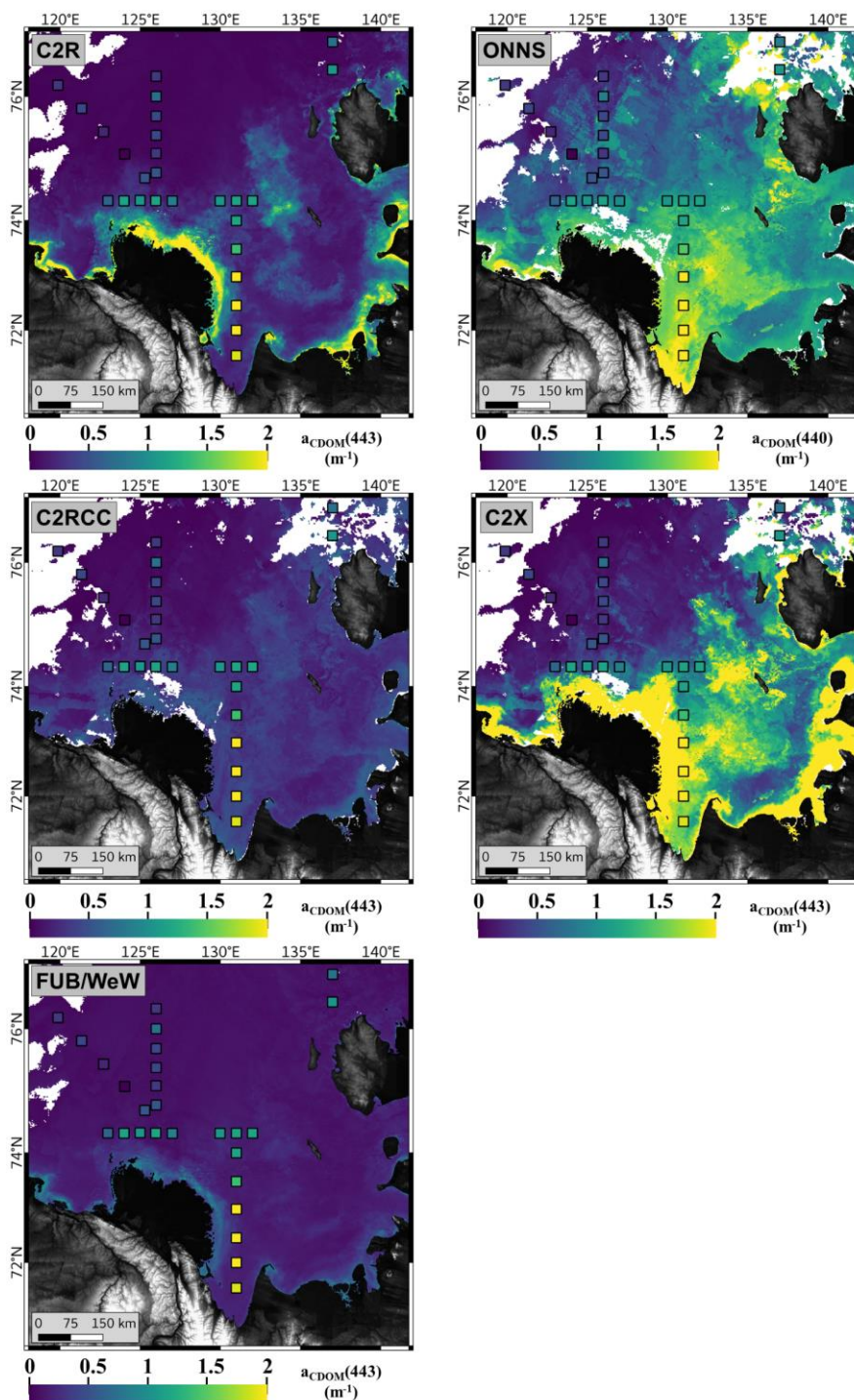
Figure 6 Surface water a_{CDOM}(\lambda)^{sat} from MERIS mosaic from 5 scenes from September 2010 (scenes listed in Table 1) for all tested OCRS algorithms (C2R, ONNS, C2RCC, C2X, FUB/WeW). Squares show in situ a_{CDOM}(443) ( a_{CDOM}(440) for ONNS) with colors according to same color scale as satellite data.
