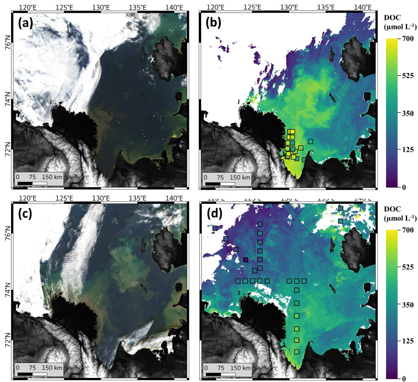
Figure 7: (a) Quasi-true color image from 5. August 2010; (b) Surface water ONNS-DOC concentration from satellite mosaics from 2010-08-03 to 2010-08-05. (c) Quasi-true color image from 7. September 2010. d) Surface water ONNS-DOC concentration from satellite mosaics from 2010-09-07 and 2010-09-18 to 2010-09-20. Squares in (b) and (d) squares indicate in situ concentrations with same color scale as satellite data.
