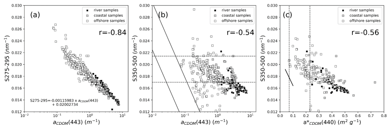
Figure 4: (a) Relationship between a_{CDOM}(443) and S_{275-295} ; (b) a_{CDOM}(443) vs. S_{350-500} with 95% confidence intervals of regressions of western Arctic coastal waters (dashed lines) and for western Arctic oceanic water (solid lines) reported by Matsuoka et al., (2011), (2012), (c) a^*_{CDOM}(440) vs. S_{350-500} with dashed lines representing the borders of a^*_{CDOM}(440) for oceanic waters report by Nelson and Siegel, (2002) and solid line shows the reported relationship between a^*_{CDOM}(440) and S_{350-500} from Matsuoka et al., (2012).
