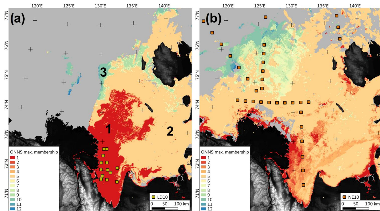
Figure C1: Optical water types from ONNS fuzzy logic classification for (a) average of 2010-08-03 to 2010-08-05 and (b) average of 2010-09-07 and 2010-09-18 to 2010-09-20
