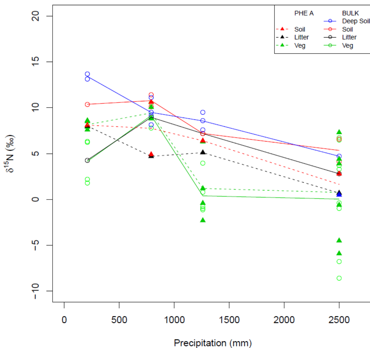
Figure 3: Patterns in isotopes of bulk material (open circles) and phea a extracts (closed triangles) from plant leaves (Veg, green), litter (black), and soil (red). Deep soils (blue) have a depth of greater than 30 cm and only a bulk isotope measurement was made for these samples. Lines connect site averages between bulk (solid) and phea a (dashed) measurements.
