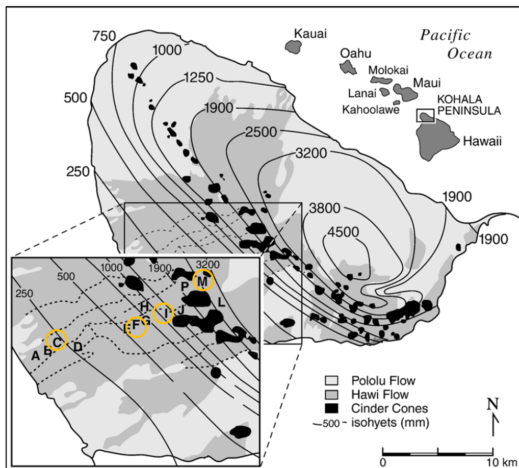
15 Figure 1: Map of Kohala climosequence sites with respect to rainfall isoclines, reproduced from Chadwick et al. (2007). Sites sampled for this study (C, F, I, and M) are circled in orange.
