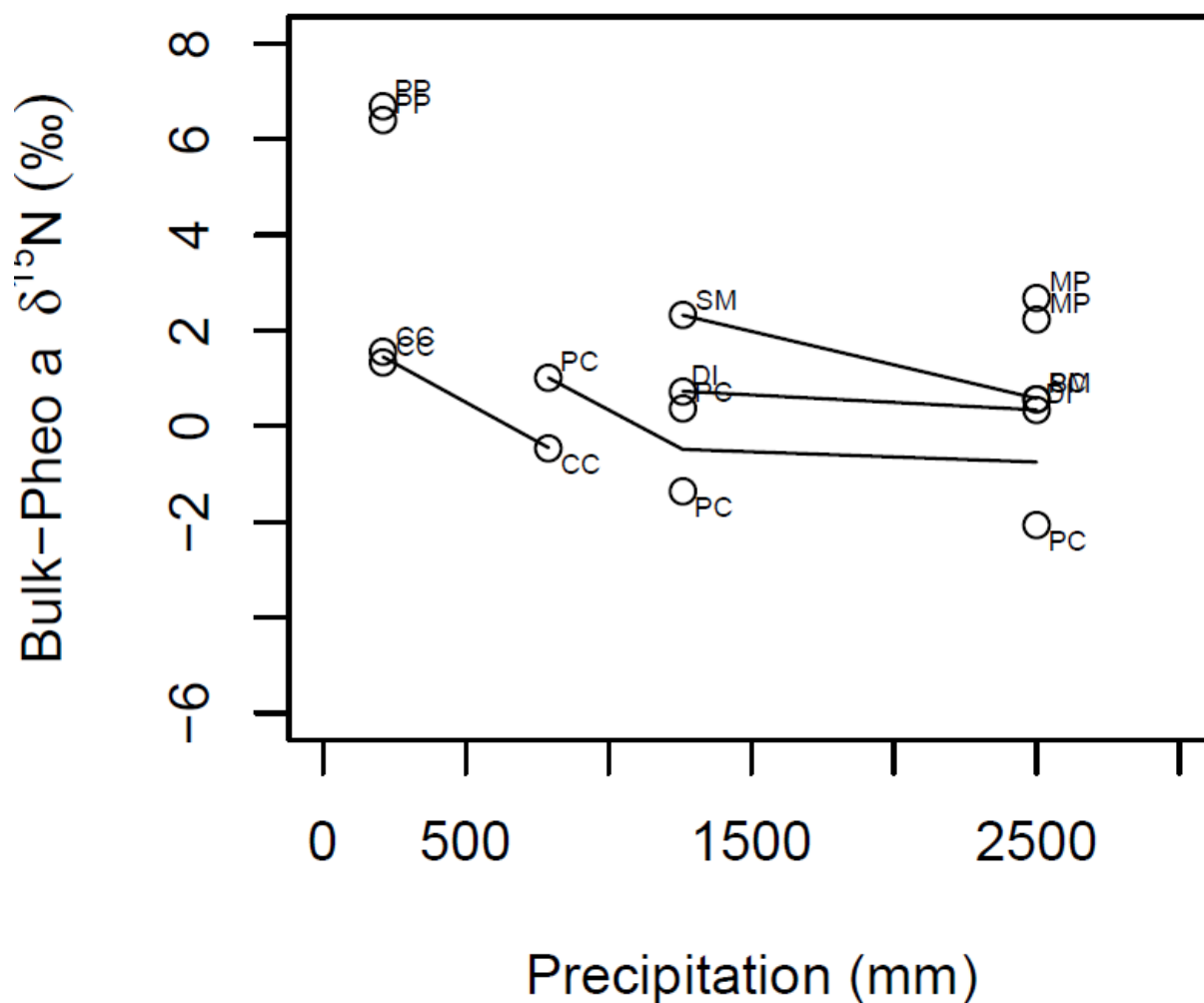
Figure 5: Comparison of species average intra-leaf \delta^{15}\text{N} offset between pheo a and bulk ( \delta^{15}\text{N}_{\text{pheo-bulk}} ) across sites. CC = C. ciliaria *, DI = D. incanum †, MP = M. polymorpha ‡, PC = P. clandestinum *, PP = P. pallida †‡, SM = S. madagascariensis . * = C4 pathway, † = N fixer, ‡ = tree
