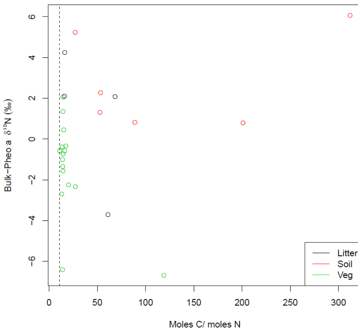
Figure 2: C/N ratios for pheo a isolates higher than 11 (dashed line) reveal contamination by carbon compounds. Effect of this contamination on pheo a \delta^{15}\text{N} is investigated by comparing “pheo a ” molar C/N with the offset between pheo a and bulk \delta^{15}\text{N} for litter (black), soil (red), and vegetation (green) samples. Lack of a systematic relationship between high C/N ratios and greater similarity of pheo a \delta^{15}\text{N} to bulk values is evidence against contamination of the pheo a samples by N from the greater bulk sample.
