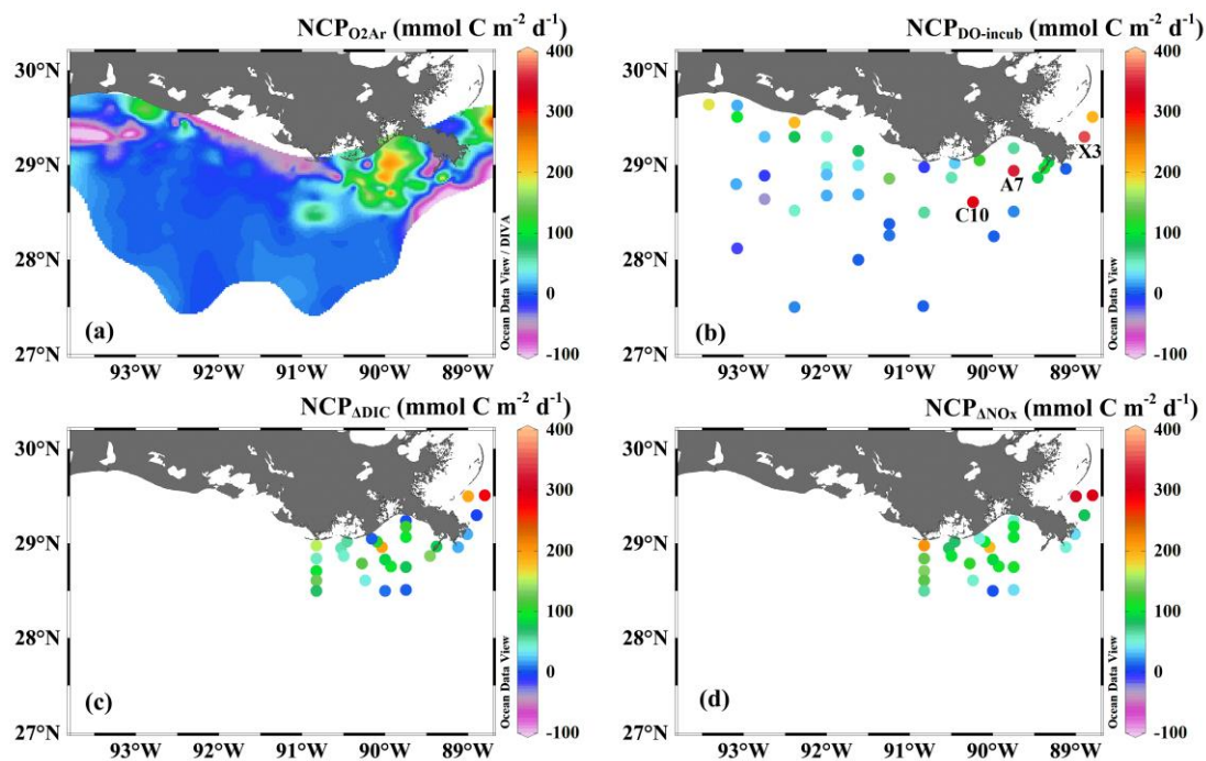
Fig. 5. The spatial variability of (a) \text{NCP}_{\text{O}_2\text{Ar}} , (b) \text{NCP}_{\text{DO-incub}} , (c) \text{NCP}_{\Delta\text{DIC}} , and (d) \text{NCP}_{\Delta\text{NO}_x} . Noted that \text{NCP}_{\Delta\text{DIC}} and \text{NCP}_{\Delta\text{NO}_x} were only estimated in the Mississippi plume (panels c, d).
