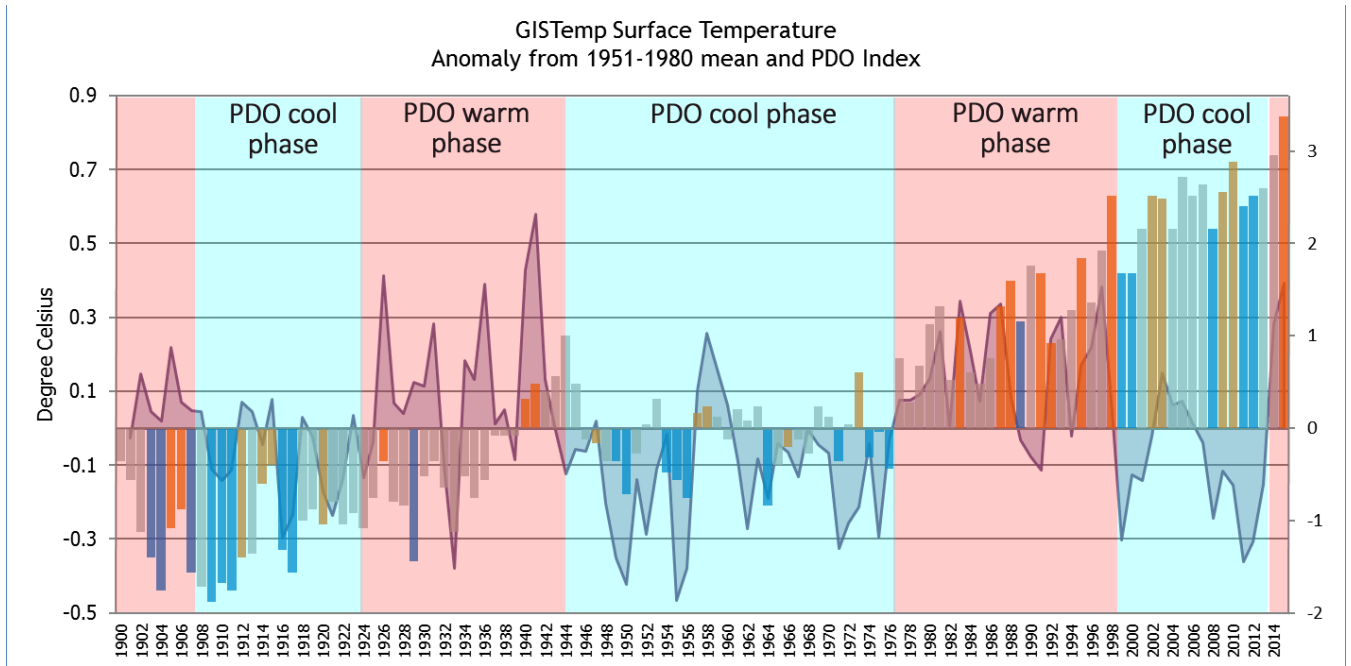
5 Figure 1. Global mean surface temperature anomaly from the 1951 to 1980 mean (GISTemp; peak of the annual bars; left scale) with La Niña years (blue bars), El Niño years (orange/brown bars) neutral years (grey bars) and the PDO index (solid line; right scale), with PDO phases marked (compiled by Miriam O'Brien for 1900 to 2015). The data sources used GISS NASA (temperature), Australian Bureau of Meteorology (ENSO years based on the Southern Oscillation Index) Japan Meteorological 10 Society (PDO index) and Trenberth 2015 (PDO phases).
