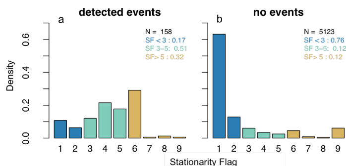
Figure 3: Stationarity flag frequency distribution of half-hourly timestamps, separating between fluxes that were influenced by events (a) and those where no events were detected (b). Stationarity flags were grouped into the three classes high (dark blue), medium (light blue) and low (light brown) stationarity. The total count of timestamps is slightly above the sum of timestamps available during the study period (5280) due to an occasional occurrence of several events in a single half-hour window.
