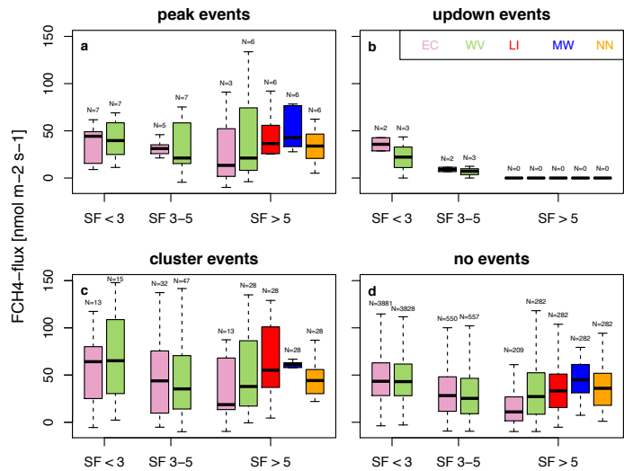
5 Figure 4: Methane fluxes based on the EC (purple) and wavelet (green) flux processing method for three stationarity flag (SF) categories during different event types at tower 2. For SF > 5, where methane fluxes based on the EC method would be excluded during the regular post-processing quality control, in addition the values for the three gapfilling methods (red: LI; blue: MW; orange: NN) are shown. For details on graph features, please refer to Figure 2 .
