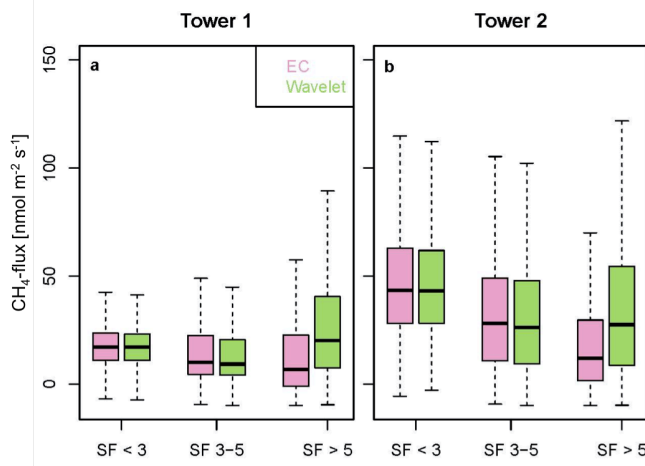
Figure 1: Median and variability of non-gapfilled methane fluxes based on the EC (purple) and wavelet (green) flux processing methods for different stationarity classes at towers 1 (a) and tower 2 (b). Black horizontal bars give the median, colored boxes indicate the interquartile range covered by the 2 nd and 3 rd quartile, while whiskers show the minimum and maximum, respectively, flux rates.
