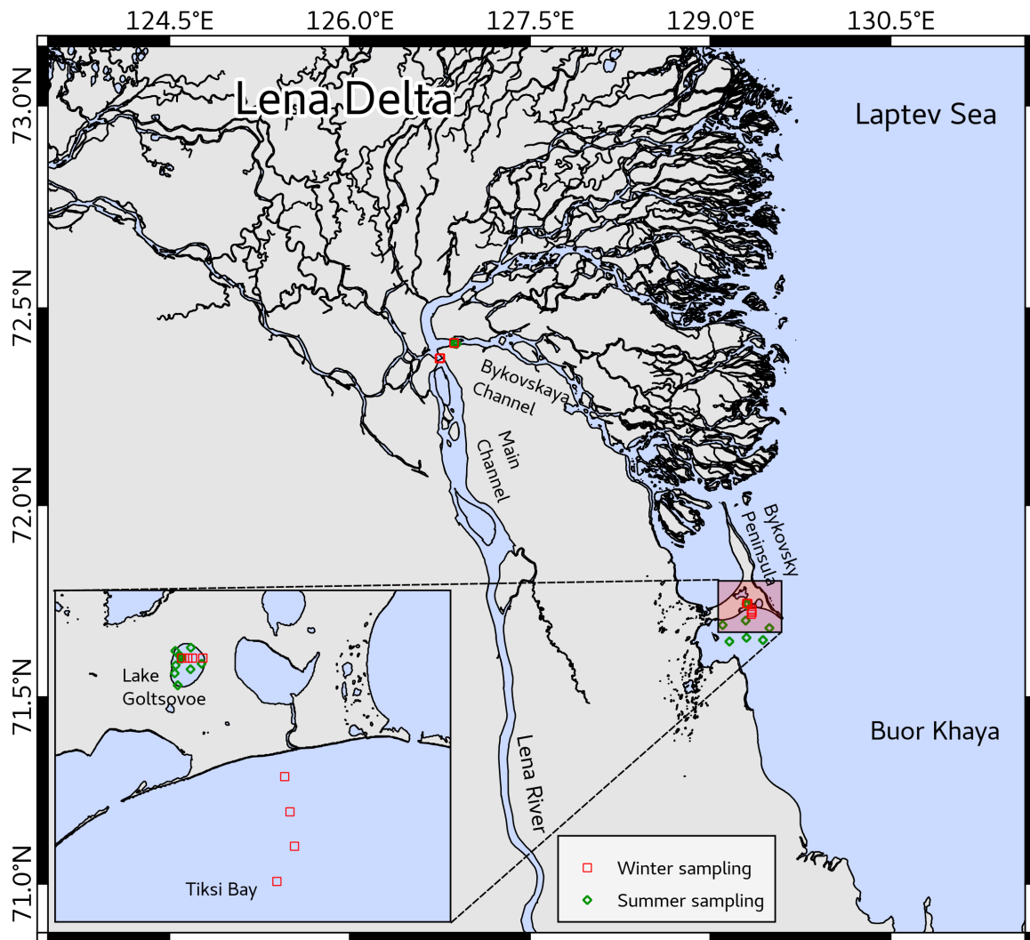
185 Figure 1: Map of the study area in the Lena River and Buor Khaya Bay (Siberia, Russia.) The inset shows details of the sampling at Lake Goltsgvoe. Sampling locations in winter are shown in red, summer sampling locations in green. Created by Bennet Juhls.
