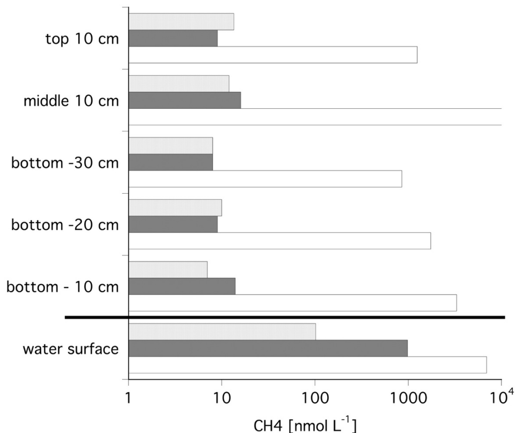
325 Figure 3: Median methane concentrations in the ice cores and in the water below the ice; Date from Tiksi Bay are shown in light grey, data for Lake Golzovoye in dark grey, with core #24 shown separately in white. Note the logarithmic scale.
