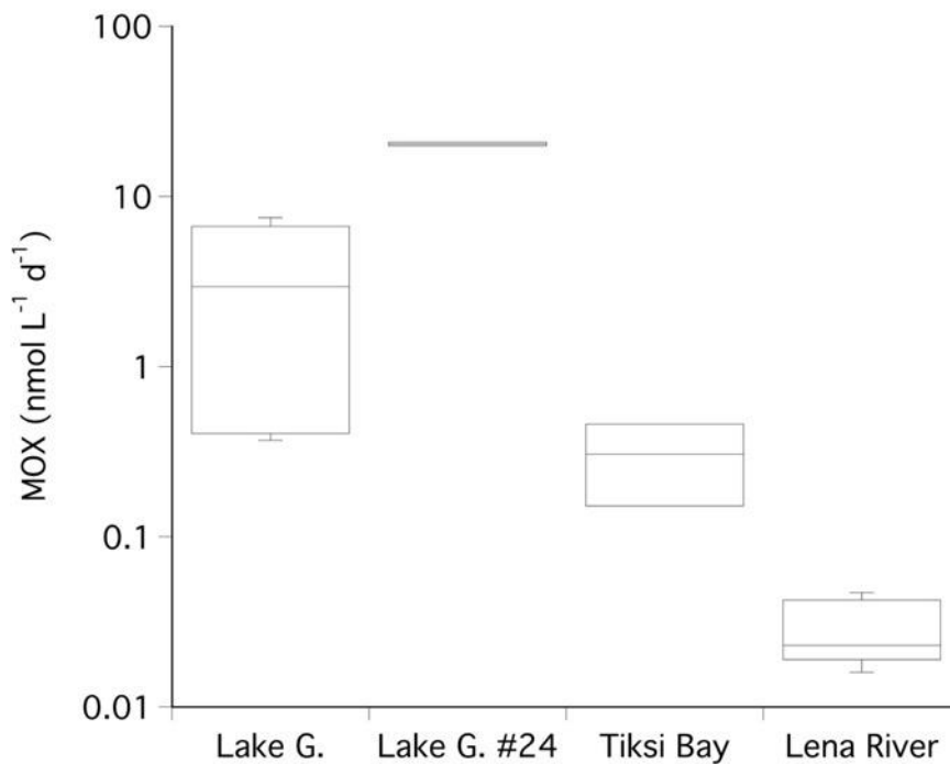
Figure 4: Box plot of the calculated methane oxidation rates (MOX) in water under ice cover at Lake Golzovoye, at the location of ice core #24, Tiksi Bay and the Lena River. Note the logarithmic scale.
