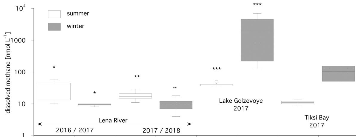
305 Figure 2: Median summer and winter methane concentrations at the Lena River, Lake Golzovoye and Tiksi Bay in the years 2016 – 2018. Bright columns indicate summer values, dark columns indicate winter values. The Asterisks indicate significant differences between summer and winter data..
