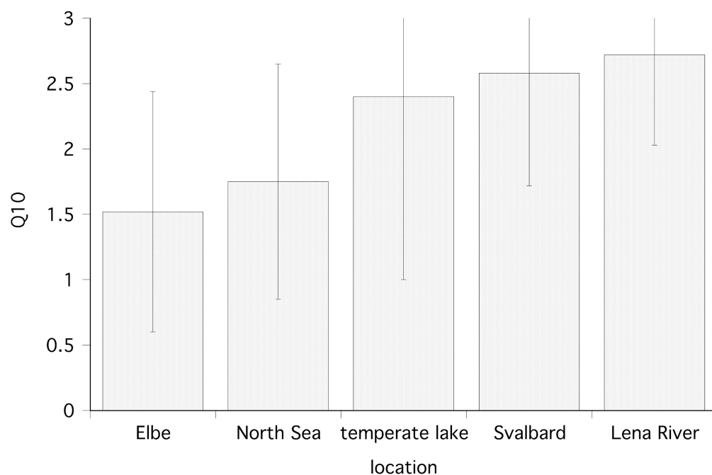
545 Figure 6: Temperature dependence ( Q_{10} ) of the methane oxidation rate at different locations; shown are the mean and standard deviation, Data for Elbe and North Sea are from Bussmann et al. (2015), data for the temperate lake are from Thottathil et al. (2019).
