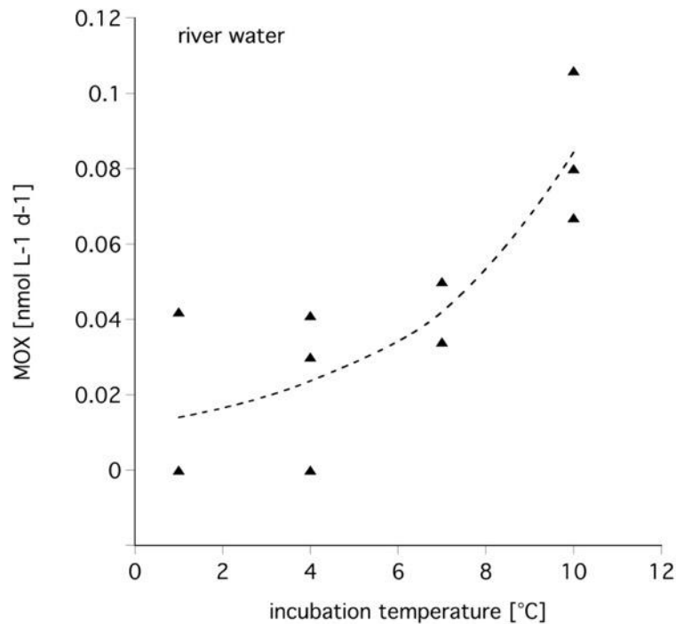
360 Figure 5: Influence of incubation temperature on methane oxidation rate for Lena River water, winter 2017.
