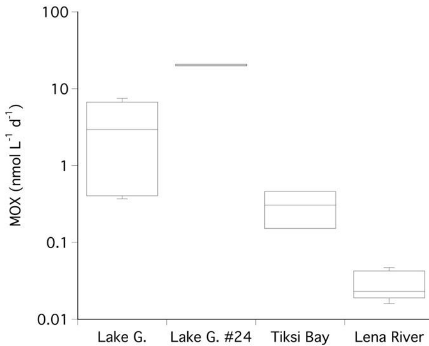
350 Figure 4: Box plot of the calculated methane oxidation rates (MOX) in water under ice cover at Lake Golzovoye, at the location of ice core #24, Tiksi Bay and the Lena River. Note the logarithmic scale.
