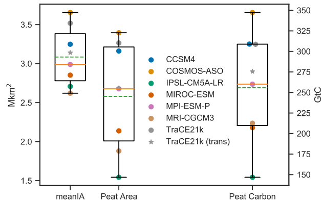
Figure 3. Spread of global annual mean inundated area (meanIA), peatland area, and peatland carbon over during the seven -LGM (21 kyr BP) in timeslices forced with climate anomalies from seven different climate models (see Sect. 2.2). The box, the solid line, and the dashed line indicate the interquartile range, the median and the mean from the seven simulations. The star indicates the values of the transient simulation for the same time period using climate anomalies from Trace21k TraCE21k .
