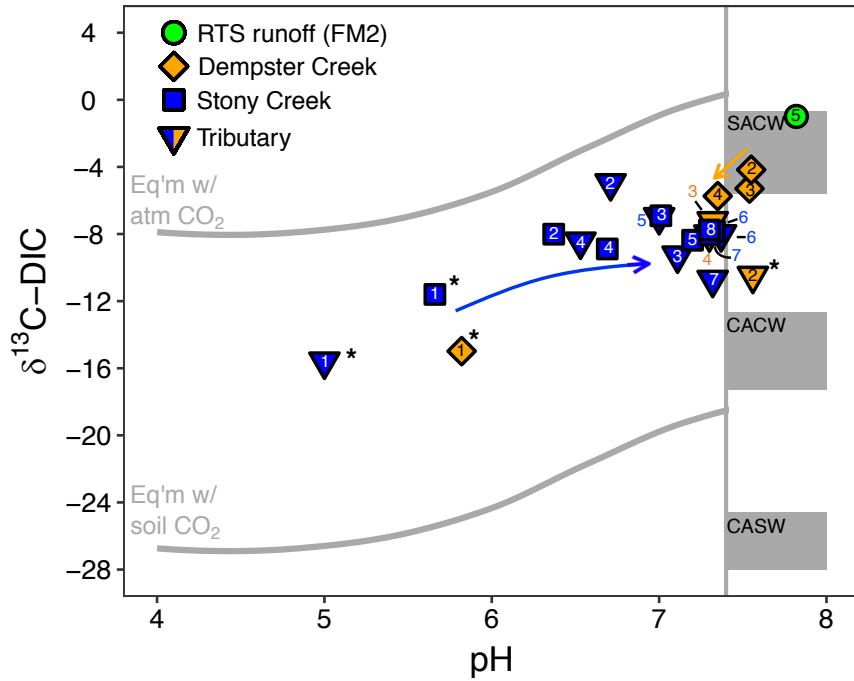
835 836 Figure 4. The pH and composition of dissolved inorganic carbon stable isotopes ( \delta^{13}\text{C-DIC} ) in streams. The upper 837 and lower reference lines depict theoretical end-members for equilibrium reactions (mixing with atmospheric and 838 biotic \text{CO}_2 , respectively). Gray boxes span theoretical end-member values for kinetically controlled mineral 839 weathering reactions (SACW = \text{H}_2\text{SO}_4 carbonate weathering, CACW = \text{H}_2\text{CO}_3 carbonate weathering, CASW = 840 \text{H}_2\text{CO}_3 silicate weathering) (see Sect. 2.4 for derivation of end-members). The vertical line corresponds to the pH at 841 which \geq 90\% of DIC is \text{HCO}_3^- , for the mean observed stream water temperature ( 11.7^\circ\text{C} ). At \text{pH} < 7.4 , \delta^{13}\text{C-DIC} 842 values primarily reflect equilibrium (rather than kinetic) controls on DIC cycling. Arrows reflect increasing 843 downstream distance from the headwaters in Stony Creek and from the first retrogressive thaw slump (RTS) 844 affected site in Dempster Creek. Site numbers given within symbols (Table A1). *Not RTS affected. 845
