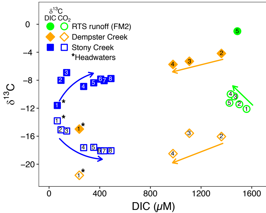
848 849 Figure 5. The composition of DIC and \text{CO}_2 stable isotopes at varying DIC concentrations along the Dempster and 850 Stony Creek mainstems, and in the rill runoff of retrogressive thaw slump (RTS) FM2. Arrows reflect increasing 851 downstream distance from headwaters in Stony Creek, from the first RTS-affected site in Dempster Creek, and from 852 the start of the FM2 runoff transect. Site numbers given within symbols (Table A1). *Site in headwaters and not 853 affected by RTSs.
