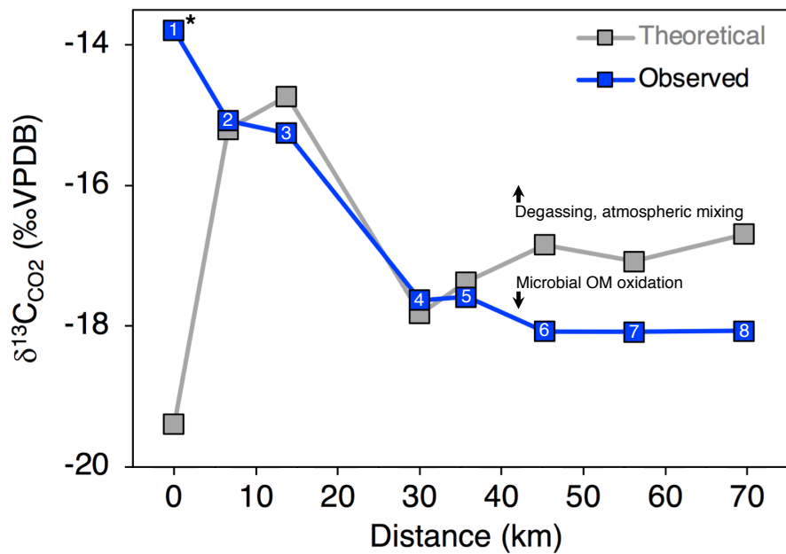
854 855 Figure 6. Observed and expected \delta^{13}\text{C-CO}_2 values along the Stony Creek mainstem. Theoretical \delta^{13}\text{C-CO}_2 values 856 were calculated as detailed in Sect. 2.6 and reflect changes in \text{CO}_2 due to DIC speciation (i.e. \text{H}_2\text{CO}_3 \rightleftharpoons \text{H}^+ + \text{HCO}_3^- , 857 Eq. 8). Deviation from theoretical \delta^{13}\text{C-CO}_2 values by observed values thus indicates isotopic effects from 858 degassing and/or microbial oxidation of organic matter (OM), as indicated by the arrows. Site numbers given within 859 symbols (Table A1). *Site was not affected by retrogressive thaw slumps.
