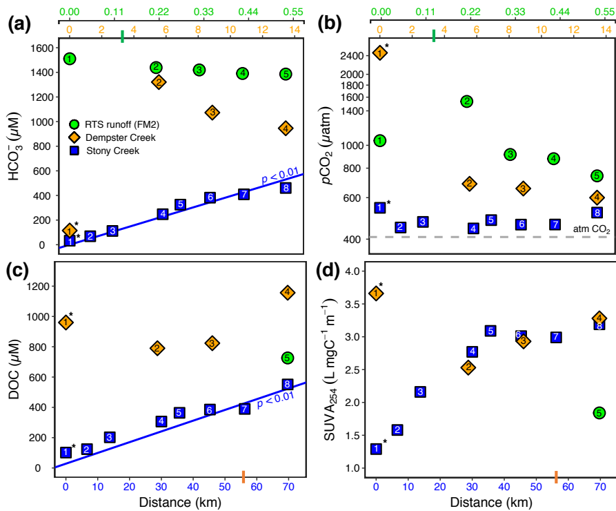
823 824 Figure 3. (a) \text{HCO}_3^- , (b) p\text{CO}_2 , (c) dissolved organic carbon (DOC), and (d) \text{SUVA}_{254} along the RTS FM2 runoff 825 FM2 runoff transect (0–0.55 km, upper x-axis), Dempster Creek (0–14 km, below RTS FM2 x-axis) and Stony 826 Creek (0–70 km, lower x-axis). For the RTS FM2 runoff, DOC and \text{SUVA}_{254} were sampled only at 0.55 km. 827 Regression lines in (a) and (c) are from a Mann-Kendall test (details in Sect. 2.7). Bars on x-axes indicate where 828 RTS FM2 runoff enters the Dempster Creek transect (3.3 km) and where Dempster Creek enters Stony Creek (56 829 km). Site numbers are given within symbols (Table A1). *Not RTS affected.
