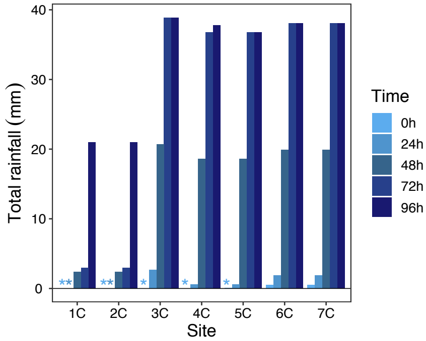
880 881 Figure A2. Total rainfall in 24 h increments preceding the sampling of each Stony Creek tributary. Rainfall data 882 were obtained from a Government of Northwest Territories weather station on the Peel Plateau located near the RTS 883 FM2. Locations of tributary sampling sites and the weather station are shown in Fig. 1. *Indicates no rainfall in the 884 24 h window.
