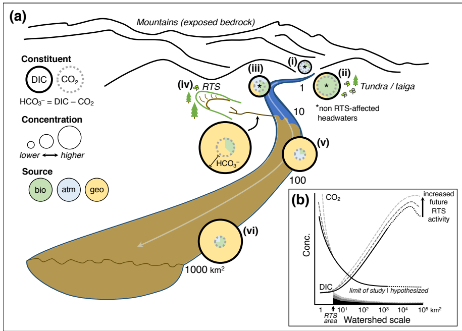
860 861 Figure 7. (a) Conceptual model of retrogressive thaw slump (RTS) activity and mineral weathering effects on 862 carbon cycling in glaciated thermokarst terrains like the Peel Plateau. Source abbreviations: bio = biogenic, atm = 863 atmospheric, geo = geogenic. (b) RTS effects on CO 2 and DIC (Σ[CO 2 , carbonate alkalinity]) observed in this study 864 (dark solid line), projected across broader scales in the modern-day (dark dotted line), and under hypothetical future 865 scenarios of increasing RTS activity (medium- and light-gray dashed lines). Shaded regions along x-axis depict 866 relative RTS area approximated for modern-day (black) and for hypothetical future increases in RTS area (medium- 867 and light-gray).
