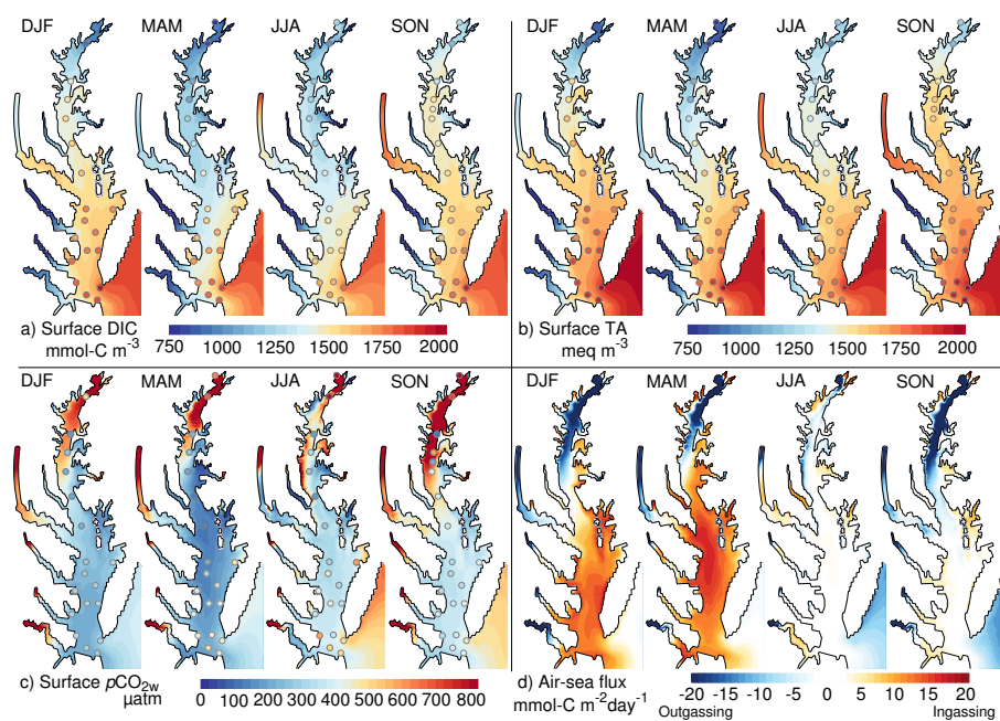
Figure 5. Overview of the spatial and seasonal variability of the inorganic carbon system. The shading represents a seasonal climatology from the Control experiment (years 2000–2014). The circles are derived from observations (see Section Methods). DJF is Dec. to Feb., MAM is March to May, JJA is June to Aug., and SON is Sep. to Nov.
