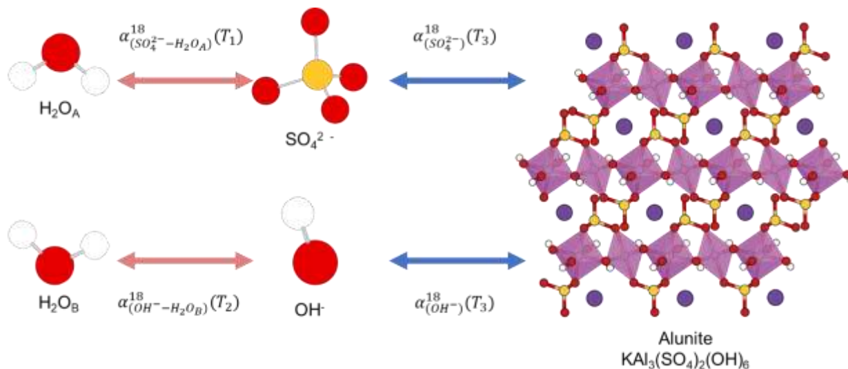
Figure 1. Sketch of alunite precipitation from water. The alunite could be a single-mineral geothermometer if three conditions are fully all satisfied: (1) \text{H}_2\text{O}_A = \text{H}_2\text{O}_B , (2) T_1 = T_2 = T_3 , and (3) all the four reactions are fully reversible and attain equilibrium. White, red, yellow, pink, and purple spheres represent hydrogen, oxygen, sulfur, aluminum, and potassium atoms, respectively.
