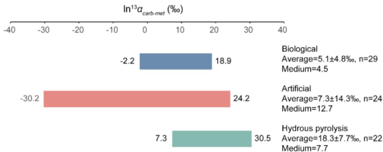
Figure 3. \ln^{13}\alpha_{carb-met} values of biological, artificial, and hydrous pyrolysis produced acetic acid.
