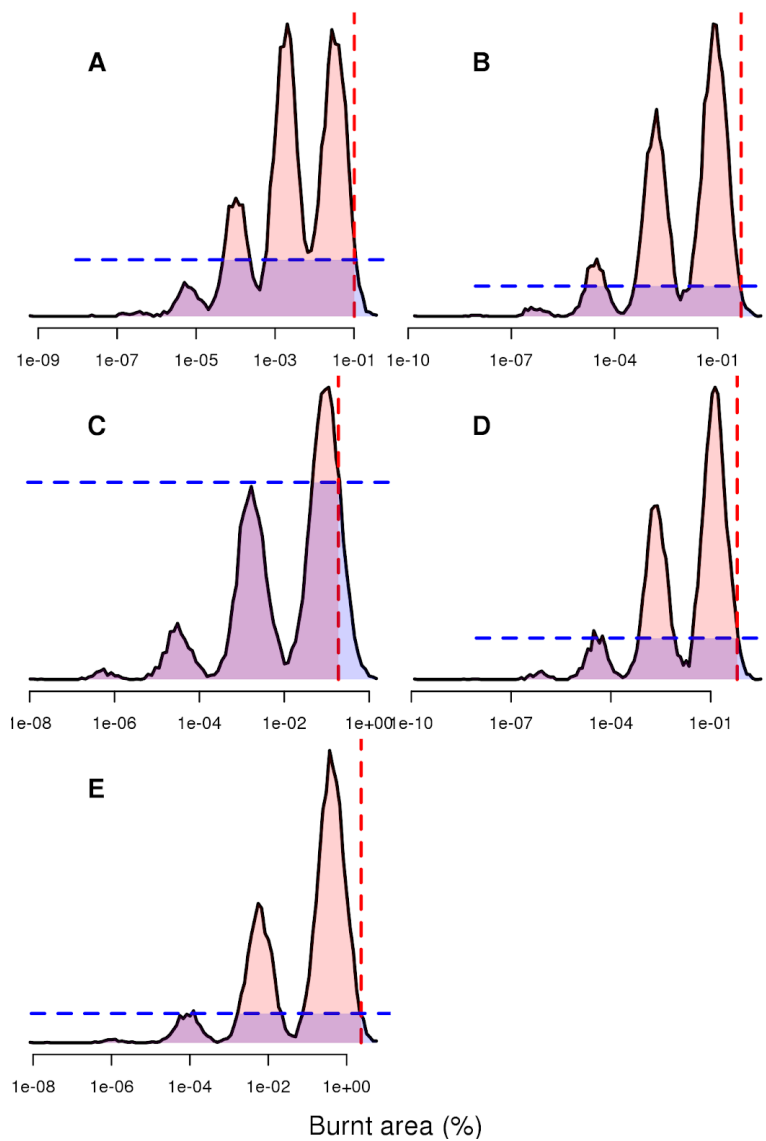
Figure B1: Full model posterior solution (black line) for August 2005 across each of the sub-regions compared to MODIS Collection 6 MCD64A1 burned area product (Giglio et al., 2018) (red dashed line). Red shaded area (posterior solution smaller than observed) shows the likelihood high burnt areas were influenced by factors external to the modelling framework. Blue shaded area is the area of the posterior which has less chance of occurrence than the observed burnt area (given by blue dashed line).
