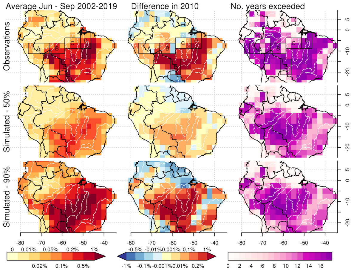
Figure C2: Same as Fig. C1 but for 2010.
