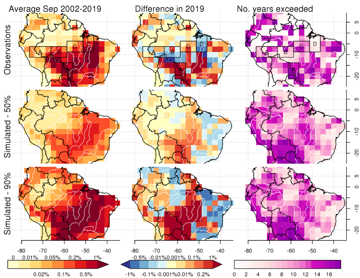
Figure 4: Same as Fig. 3 but for September.
