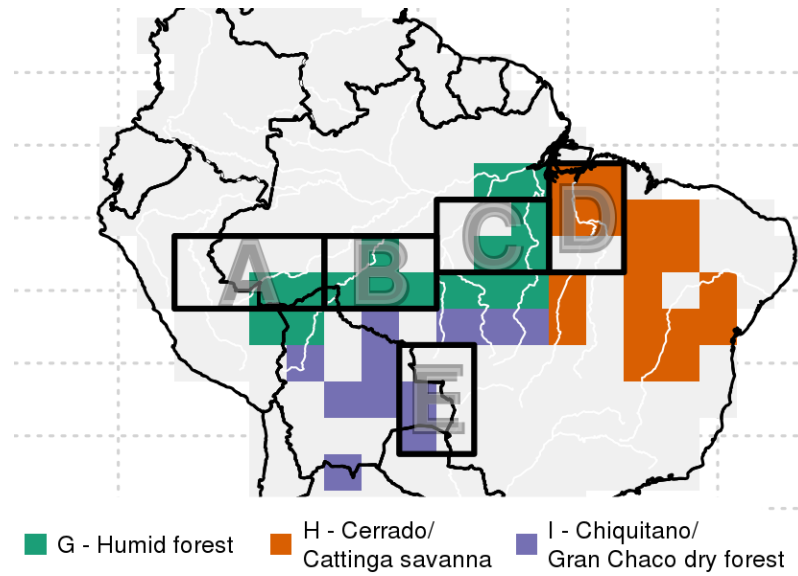
Figure A2: Study regions. Boxes mark areas used for time series in Fig 1 and rows A-E in Table 1. Coloured areas for time series if Fig 2 and F-I in Table 1, with the entire coloured region being used for F AAD. See Fig. S4 for construction of AAD and areas G-I.
