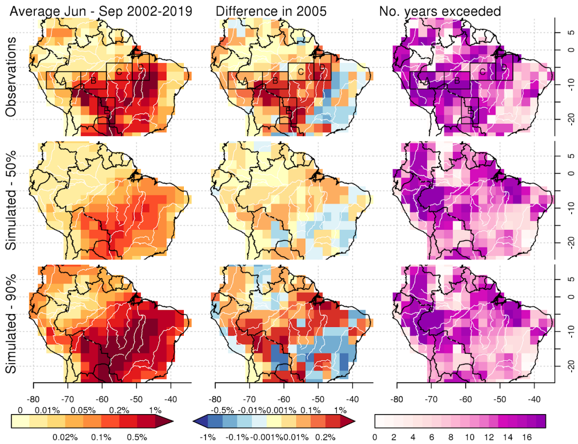
620 Figure C1: Same as Fig. 3 but for June-September annual average compared to 2005.
