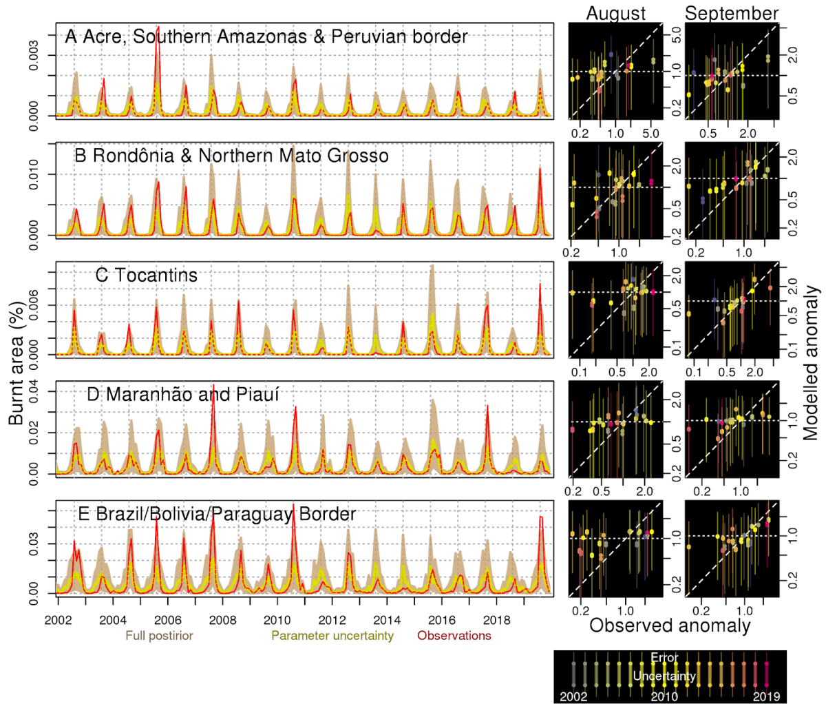
570 Figure 1: Time series and fire season anomalies for modelled and observed burnt area. See Fig. A2 for locations of A-E. Red lines show monthly burnt area observations from MCD64A1, yellow shows model accounting for parameter uncertainty (10-90%) and brown shows full model uncertainty (10-90%). The red line is dashed when observations and model accounting for parameter uncertainty overlap. Vertical grid lines are positioned for August each year. Right-hand plots show observed (x-axis) and modelled (y-axis) anomaly, calculated as 2019 burnt area over 575 2002-2019 climatological average burnt area for (first column) August and (second column) September. The colour indicates the year, with 2019 in red. Thin lines show 10-90% full model uncertainty, while dots and thick line indicate 10-90% parameter uncertainty
