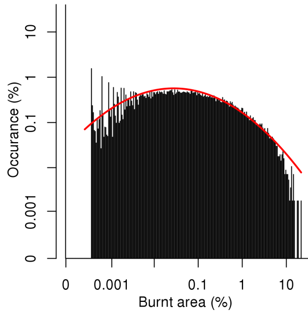
Figure A1: Distribution of burnt areas in MODIS Collection 6 MCD64A1 burned area product (Giglio et 600 al., 2018) and (red line) fitted normal distribution of logit transformed burnt areas greater than 0.
