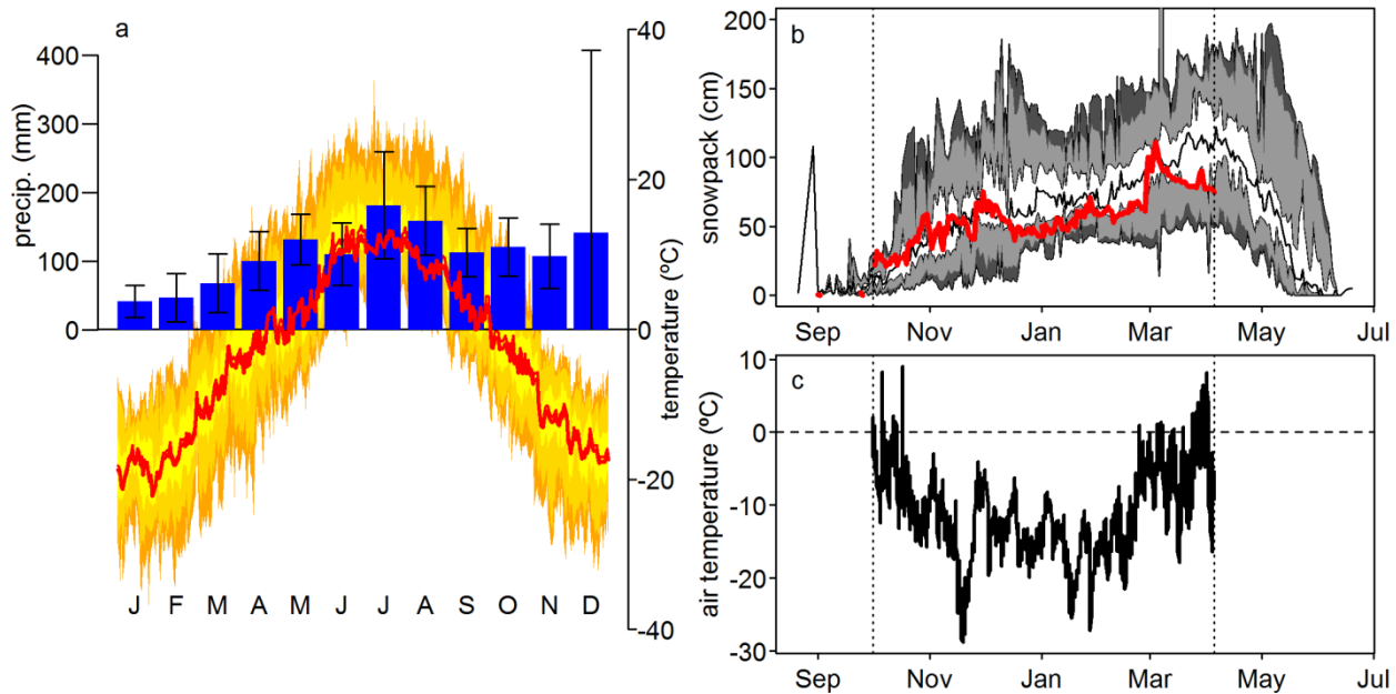
90 Figure 2. Records at Olenya Rechka meteorological station. a: Climograph (1 February 2005 - 30 April 2019). The median yearly precipitation was 1242.975 mm, with a winter (2 nd October to 5 th April) and summer precipitations of 464.95 mm and 778.025 mm, respectively. Temperature: median (red), interquartile range (yellow band), 5 th to 25 th percentiles and 75 th to 95 th percentiles (lower and upper golden bands), below the 5 th percentile and above the 95 th percentile (lower and upper orange bands). b: Snowpack thickness (2005-2017): median (black), interquartile range (white band), 5 th to 25 th percentiles and 75 th to 95 th percentiles (lower and upper light gray bands), below the 5 th percentile and above the 95 th percentile (lower and upper dark gray bands). The red line corresponds to the 2016-2017 snowpack thickness record until the snow sampling date. c: Air temperatures measured all the 3 hours during the time period when analysed snowpacks were laying on their respective locations (2016-17).
