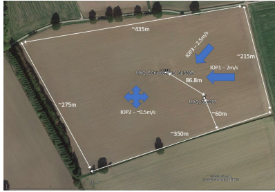
Figure 1. Scintillometer transmitter and receiver locations in relation to the dimensions of the CloudRoots field. The blue arrows indicate the wind-direction on the 3 IOPs with the wind-speed at z=2m .
