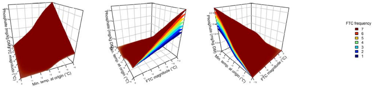
330 Figure 3: Phosphate concentrations depended on the three-fold interactive effects of winter climatic origin (expressed as 331 longterm mean minimum winter temperature at the origin), FTC magnitude (expressed as the minimum temperature 332 experienced during the FTC manipulation and displayed for freezing temperatures) and FTC frequency during the FTC 333 manipulation. FTC = freeze-thaw cycle. The four dimensional representation is displayed from three different angles (see 334 Appendix D for an animated version) and is based on the best model fit in the hierarchical regression analysis (model 15. in 335 Table 5 with coefficients a_1 = 0.49455 ; a_2 = 0.01253 ; a_3 = 1.37580 ; a_4 = 0.00890 ; a_5 = 0.00217 ).
