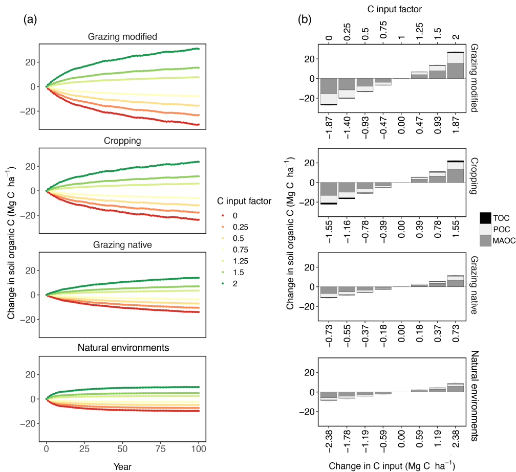
Figure 5. (a) The 100-year simulations showing the changes in total organic C (TOC) in the topsoil (0–0.3 m) following changes in C input ( n = 4,043 ). At each site, baseline C input was multiplied by the factor 0, 0.25, 0.5, 0.75, 1.25, 1.5, and 2 to derive different C input levels. (b) Median changes in TOC and its fractions, consisting of the particulate and mineral-associated organic C (POC and MAOC), calculated over the last 11 years of the simulation (at the new or near new equilibrium).
