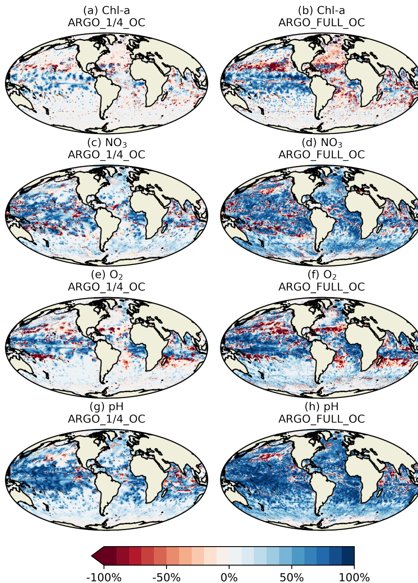
Figure 10. MAE red_% over OC for Chl- a , NO 3 , O 2 , pH for December 2009 at 100 m depth.
