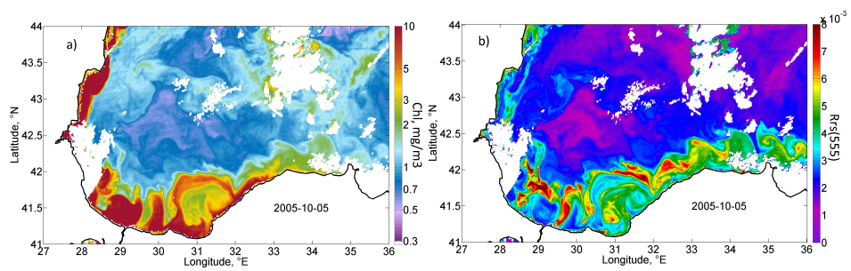
Fig. 4. Figure R4. MODIS daily map of Chl (a) and Rrs (b) for 5 October 2005 illustrating the initial growth of coccolithophores on the front of the rich in Chl plume waters
