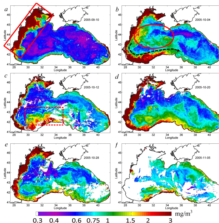
Fig. 1. Figure R1: 8-daily maps of chlorophyll-a concentration, mg m -3 , centered at (a) 10 September 2005, the red rectangle (solid line) shows the Danube plume; (b) 4 October 2005, the red oval shows the phy
