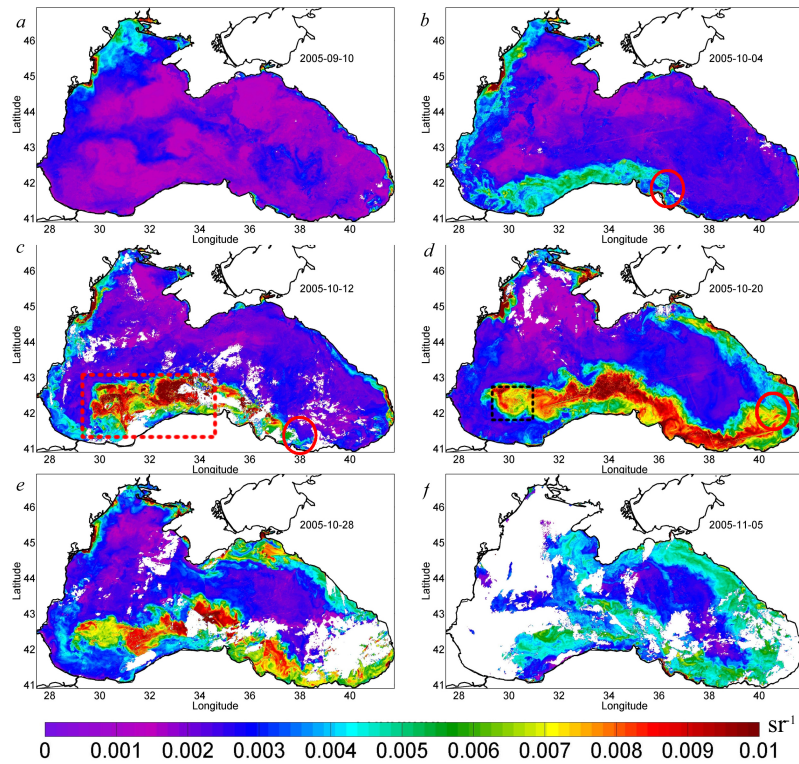
Fig. 3. Figure R3: 8-daily maps of remote sensing reflectance R_{rs} , sr^{-1} , centered at (a) 10 September 2005; (b) 4 October 2005; (c) 12 October 2005, the red rectangle shows a mixing area; (d) 20 October 2005,
