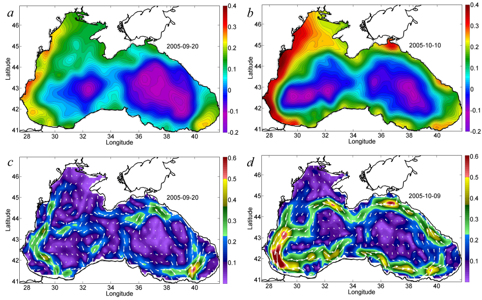
Fig. 2. Figure R2. Sea level, m: a – September 20, 2005, b – October 10, 2005; flow velocity, m/s: c – September 20, 2005, d – October 9, 2005
