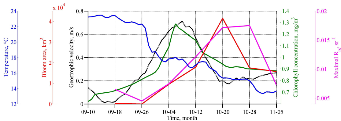
Fig. 2. R2. Average variability of SST (blue line), Rrs (purple), Chl (green) in the center of the western cyclonic cycle area of coccolithophore bloom (red) in the sea, geostrophic velocity, m/s
