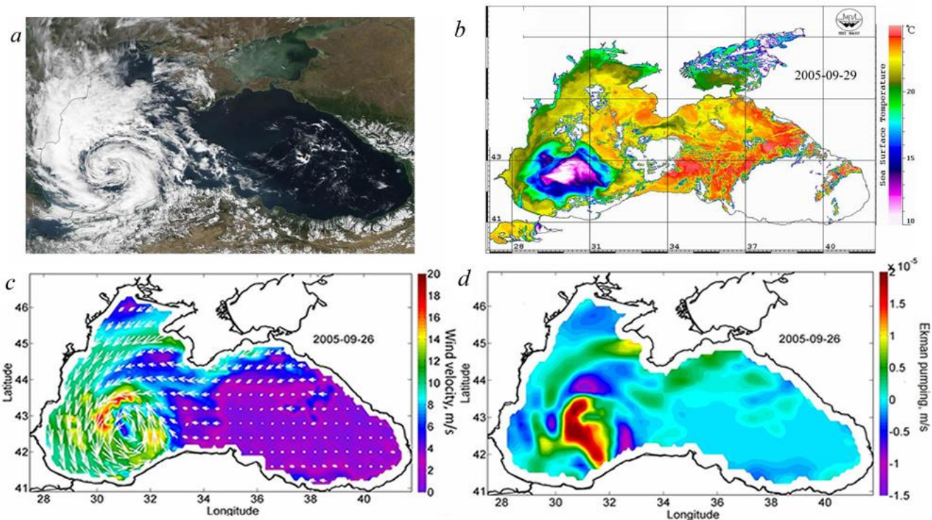
Figure 1: (a) – satellite image of MODIS-Aqua in the visible range for 27 September 2005 (data obtained from the Worldview portal); (b) – AVHRR SST (°C) for 29 September 2005; (c) – wind velocity ( \text{m s}^{-1} ) of the scatterometer SeaWinds of the satellite QuikSCAT on 26 September 2005; (d) – ekman pumping velocity ( \text{m s}^{-1} ) on 26 September 2005, calculated from QuikSCAT data ( positive values - the velocity is directed upwards ).
