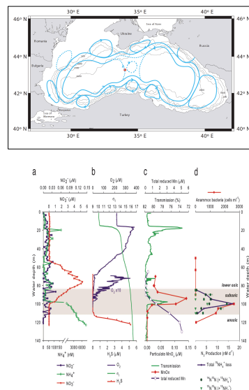
Fig. 1. Vertical distribution of inorganic nitrogen (a), \text{O}_2 and sulfide (b), light transmission, particulate \text{MnO}_2 and total reduced Mn (c), and ammonia bacterial abundance and ^{15}\text{N}_2 production rates (d).
