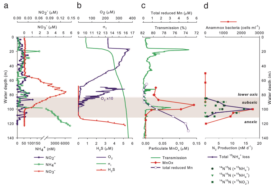
Fig. 1. Vertical distribution of inorganic nitrogen (a), \text{O}_2 and sulfide (b), light transmission, particulate \text{MnO}_x , and total reduced Mn (c), and anammox bacterial abundance and ^{15}\text{N}_2 production rates (d).
