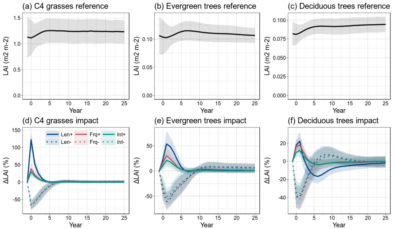
340 Figure 7. Response of the vegetation to the different rainfall scenarios for the Dahra site, in function of years since the disturbance event. (a-c) reference LAI of each PFT, averaged over all ensemble members; (d-f) vegetation response as the mean relative LAI difference between the scenario runs and the reference runs. Shaded areas indicate variability of the model runs over all ensemble members ( \pm 1\sigma ).
