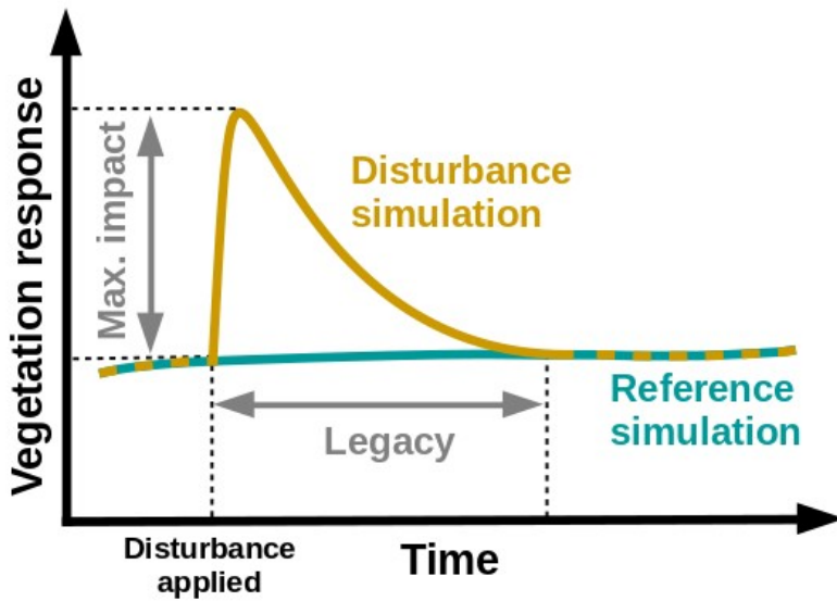
260 Figure 4. Concept of the model experimental setup, consisting of a disturbance simulation in which a rainfall disturbance is applied and a reference run, which is based on the same meteorological drivers but without any disturbance applied. Vegetation impact is described by maximum impact (amplitude) and legacy (years). The average impact is derived by subtracting the output of the reference simulations from the output of the disturbance simulations for each ensemble member, and then taking the average of the result over all ensemble members. The legacy is calculated as the last year for which the 265 average impact is larger than its standard deviation.
