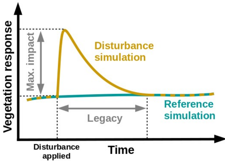
225 Figure 4. Concept of the model experimental setup, consisting of a disturbance simulation in which a rainfall disturbance is applied and a reference run, which is based on the same meteorological drivers but without any disturbance applied. Vegetation impact is described by maximum impact (amplitude) and legacy (years). The average impact is derived by subtracting the output of the reference simulations from the output of the disturbance simulations for each ensemble member, and then taking the average of the result over all ensemble members. The legacy is calculated as the last year for which the 230 average impact is larger than its standard deviation.
