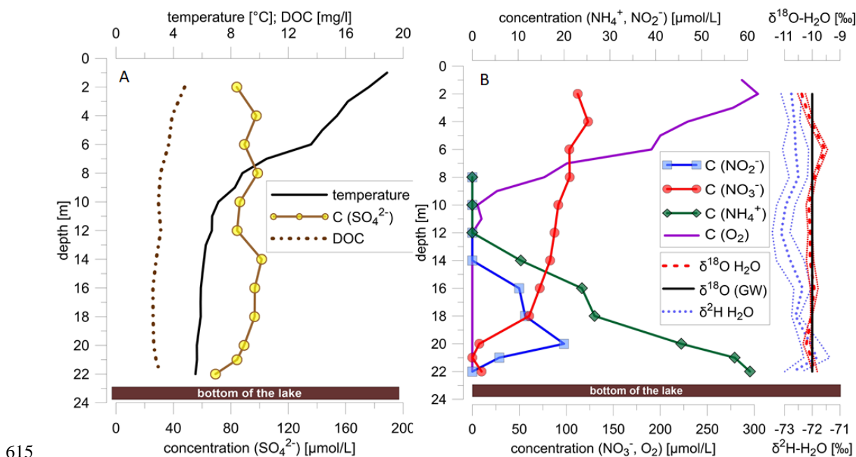
Figure 1A and B. Temperature profile and vertical distribution of concentrations of DOC, sulfate (left) and (B) dissolved nitrate, nitrite, ammonium, and dissolved oxygen, \delta^2\text{H} and \delta^{18}\text{O} values of lake water and \delta^{18}\text{O} value of groundwater (GW) (right).
