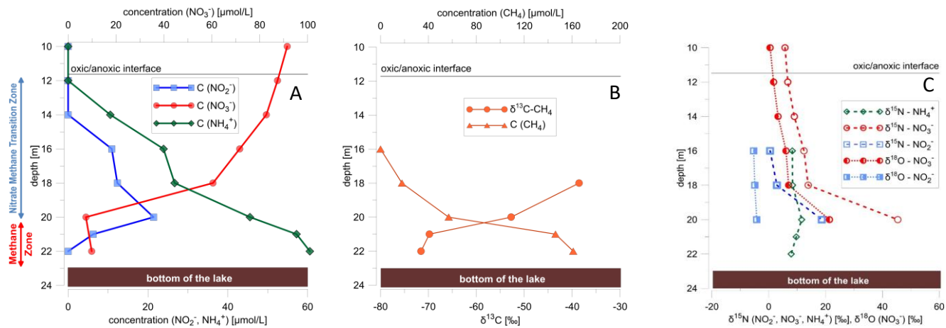
Figure 2A-C. Water column profiles below the oxycline (10 to 22 m) for methane, nitrate, nitrite and ammonium concentrations and (B) stable isotope data and concentration profile of methane ( \delta^{13}\text{C} ), and (C) nitrate ( \delta^{15}\text{N} , \delta^{18}\text{O} ), nitrite ( \delta^{15}\text{N} , \delta^{18}\text{O} ), and ammonium ( \delta^{15}\text{N}_{\text{NH}_4} ) isotopes.
