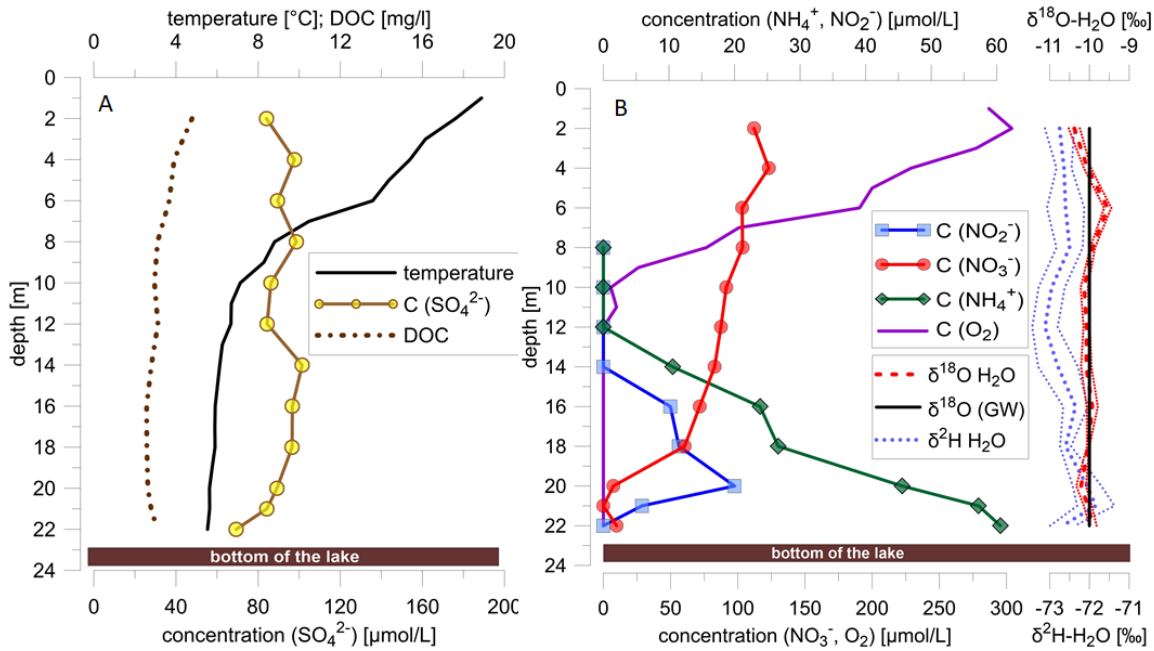
610 Figure 1A and B. Temperature profile and vertical distribution of concentrations of DOC, sulfate (left) and (B) dissolved nitrate, nitrite, ammonium, and dissolved oxygen, δ 2 H and δ 18 O values of lake water and δ 18 O value of groundwater (GW) (right).
