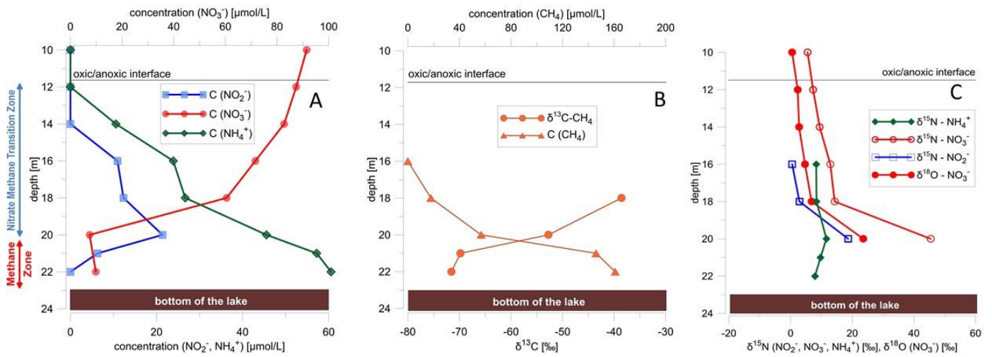
620 Figure 2A-C. Water column profiles below the oxycline (10 to 22 m) for methane, nitrate, nitrite and ammonium concentrations and (B) stable isotope data and concentration profile of methane ( \delta^{13}\text{C} ), and (C) nitrate ( \delta^{15}\text{N} , \delta^{18}\text{O} ), nitrite ( \delta^{15}\text{N} , \delta^{18}\text{O} ), and ammonium ( \delta^{15}\text{N}_{\text{NH}_4} ) isotopes. \delta^{15}\text{N} and \delta^{18}\text{O} values of nitrate were calculated by mass-weighted isotope mass balance calculation using a \delta^{18}\text{O} value for nitrite of +4‰ (Casciotti et al., 2007).
