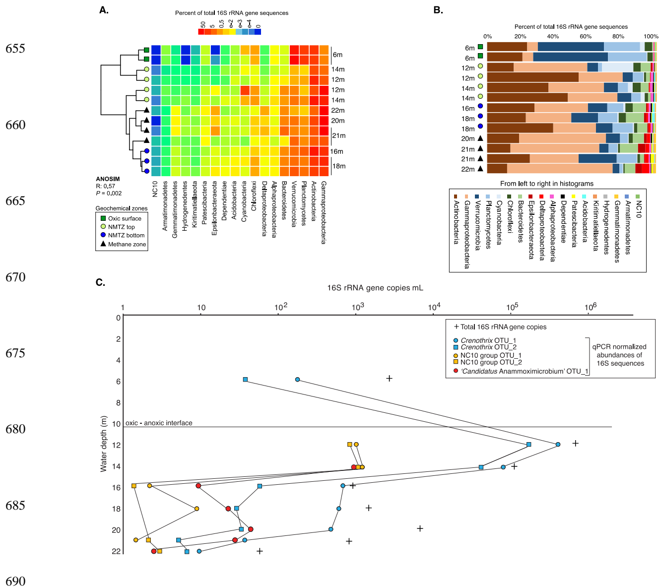
Figure 3A-C. Analysis of 16S rRNA gene data from microbial communities in the stratified lake. (A) Heatmap showing the relative abundance of specific groups in the 16S rRNA gene sequencing data, and corresponding hierarchical clustering analysis (analysis of similarity (ANOSIM) P value = 0.002) of four geochemically defined zones. For those depths where replicates were obtained, the data for both replicates are shown.
