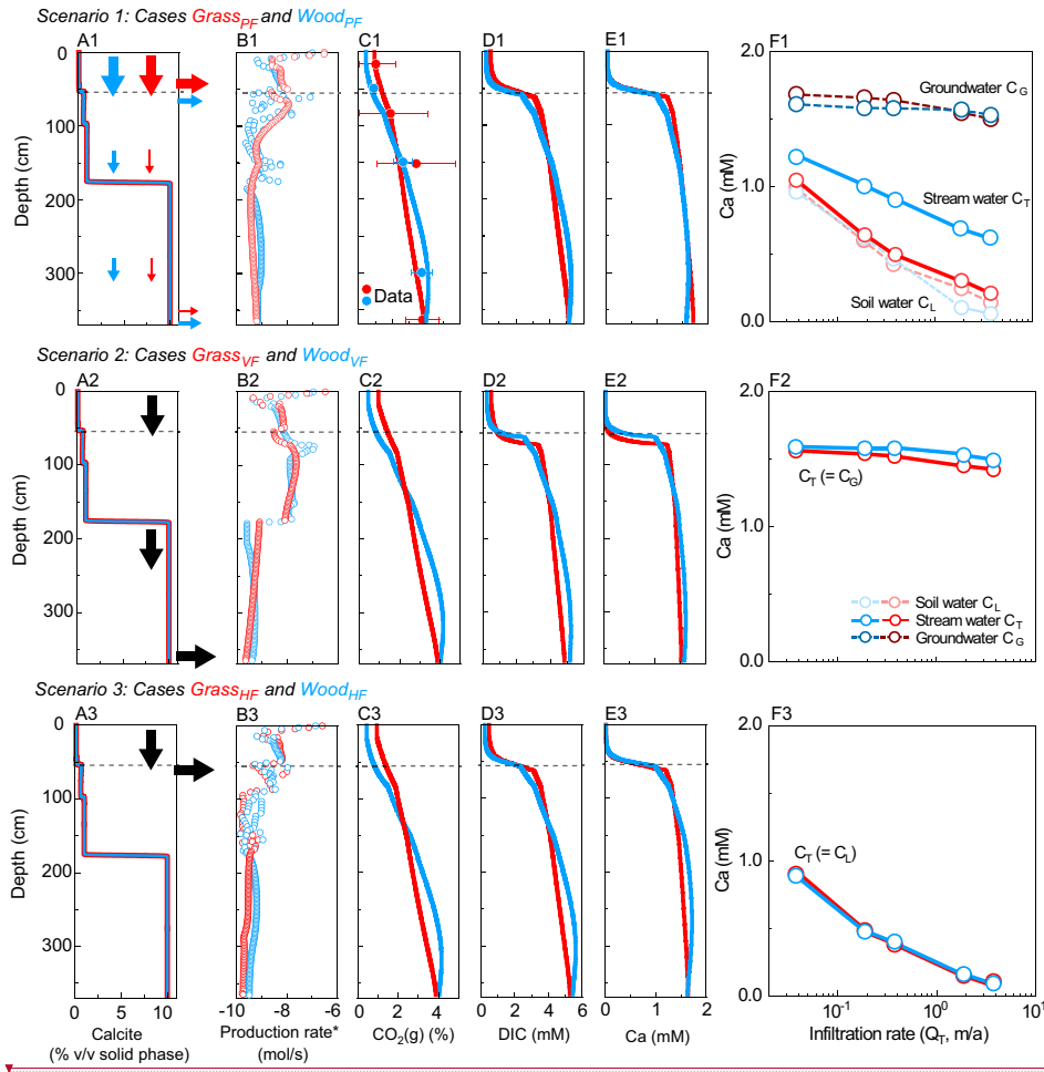
Figure 3. Simulated depth profiles of (A) calcite (vol %), (B) soil \text{CO}_2 production rate; (C) \text{CO}_2(\text{g}) (%), (D) DIC, and (E) Ca at 0.37 \text{ m/a} , and (F) effluent Ca concentrations at different infiltration rates. From top to bottom rows are Scenario 1 (Grass PF and Wood PF ; with flow partitioning, first row), Scenario 2 (Grass VF and Wood VF ; 100 % vertical flow, second row), and Scenario 3 (Grass HF and Wood HF ; 100 % lateral flow, last row). Red and blue colors present grassland and woodland, respectively. Lines and empty circles represent modelling outputs while filled circles with error bar in Figure C are the annual average \text{CO}_2(\text{g}) data (in Table 2). Arrows in Figure A indicate flow conditions. In F, soil water and groundwater refer to concentrations at the lateral (50 cm) and vertical (366 cm) outlets, respectively. Higher fractions of vertical flow in Wood PF led to higher stream Ca concentration compared to Grass PF . In Scenarios 2 and 3 without
