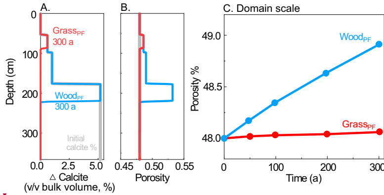
Figure 5. Predicted soil profiles of (A) calcite volume change ( \Delta\text{Calcite} = initial calcite volume - current calcite volume) and (B) porosity after 300 years; (C) Predicted temporal evolution of domain-scale porosity in the grassland and woodland. The infiltration rate is 0.37 m/a. Red and blue line represents the case GrassPF and WoodPF, respectively.
