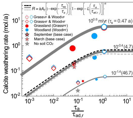
Figure 6. Calcite weathering rate as a function of the reactive time ratio \frac{\tau_a}{\tau_{ad,r}} , a proxy of the older, reactive water fraction compared to the total water fluxes . Symbols are rates from numerical experiments. Grey lines are predictions from the rate law equation at \alpha = 0.8 (Wen and Li, 2018). Large to small dots and thick to thin lines are for infiltration rates from 10^{0.6} to 10^{-1.4} m/a. The red filled stars represent the monthly rates in September (highest soil \text{CO}_2 ) and March (lowest soil \text{CO}_2 ) in the base case at 10^{-0.4} (0.37) m/a; the black to grey dash lines represent predictions with increasing soil \text{CO}_2 level (i.e., larger \tau_{eq} ) from Eq. (1). Grey filled star is for the case without soil \text{CO}_2 . At any specific infiltration rate or \tau_a , the VF and HF cases bracket the two ends whereas the PF cases fall in between. The Wood PF case with deeper roots enhanced the \text{CO}_2 -water-calcite contact (i.e., larger \frac{\tau_a}{\tau_{ad,r}} ratios), leading to higher calcite weathering rates compared to grasslands. The differences of weathering rates induced by different soil \text{CO}_2 level were relatively small compared to those hydrological changes induced by rooting depth.
