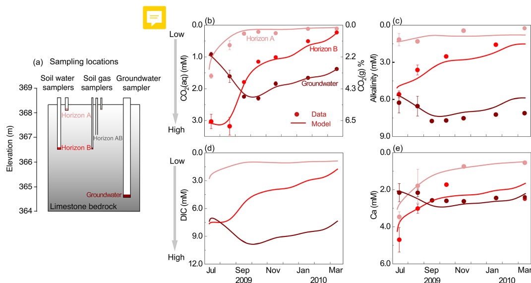
Figure 2. (a) Schematic representation of sampling depths in the Konza grassland; corresponding monthly dynamics of (b) CO 2 (aq) and CO 2 (g), (c) alkalinity, (d) DIC, and (e) Ca concentrations. Lines represent modeling outputs at the corresponding sampling depth of monthly field measurements (dots), including soil water at horizons A (16 cm) and B (152 cm), as well as groundwater (366 cm). The lines of CO 2 (aq) and CO 2 (g) in panel (b) overlapped. Note that there are no DIC data so no dots in panel (d). The temporal trends of alkalinity, DIC, and Ca mirrored those of soil CO 2 , indicating its predominant control on weathering. Note that concentrations on y axis from (b–e) are low to high, to be consistent with the layout in panel (a) with deeper water chemistry showing up deeper. TS7
