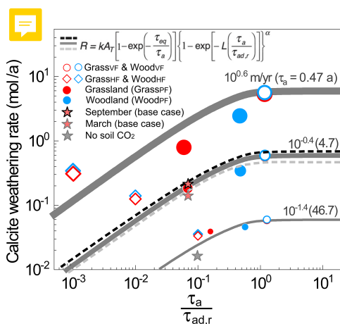
Figure 6. Calcite weathering rate as a function of the reactive time ratio \frac{\tau_a}{\tau_{ad,r}} , a proxy of the older, reactive water fraction compared to the total water fluxes. Symbols are rates from numerical experiments. Gray lines are predictions from the rate law equation at \alpha = 0.8 (Wen and Li, 2018). Large to small dots and thick to thin lines are for infiltration rates from 10^{0.6} to 10^{-1.4} m/a. The red filled stars represent the monthly rates in September (highest soil \text{CO}_2 ) and March (lowest soil \text{CO}_2 ) in the base case at 10^{-0.4} (0.37) m/a; the black to gray dashed lines represent predictions with increasing soil \text{CO}_2 level (i.e., larger \tau_{eq} ) from Eq. (1). The gray filled star is for the case without soil \text{CO}_2 . At any specific infiltration rate or \tau_a , the VF and HF cases bracket the two ends, whereas the PF cases fall in between. The WoodPF case with deeper roots enhanced the \text{CO}_2 –water–calcite contact (i.e., larger \frac{\tau_a}{\tau_{ad,r}} ratios), leading to higher calcite weathering rates compared to grasslands. The differences of weathering rates induced by different soil \text{CO}_2 level were relatively small compared to those hydrological changes induced by rooting depth.
