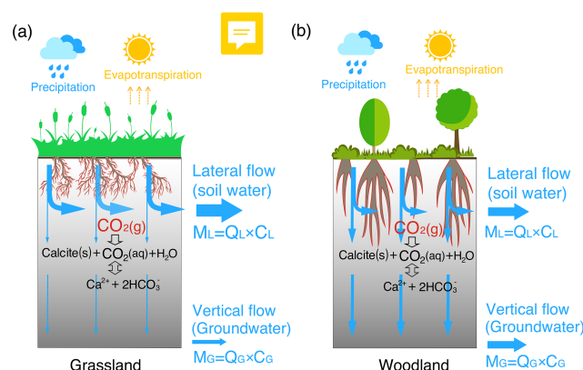
Figure 1. A conceptual diagram of hydro-biogeochemical interactions in the grassland (a) and woodland (b). The shallow and dense fine roots in the grassland promote lateral macropore development and lateral water flow. In contrast, the woodlands induce vertical macropore development that supports vertical flow (recharge) into the deep, calcite-abundant subsurface compared to the grassland. The gray color gradient reflects the calcite abundance with more calcite in depth. M_L and M_G with a unit of moles per year ( \text{CE2} ) ( = \text{flow rate } Q \text{ (m/a)} \times \text{species concentration } C \text{ (mol/m}^3) \times \text{unit cross-section area (m}^2) ) represent mass fluxes from lateral flow (soil water) and from vertical flow into groundwater, respectively. Soil water and groundwater were assumed to eventually flow into stream, where infiltration rate Q_T = Q_L + Q_G is the same as discharge that accounts for both lateral and vertical water flow.
