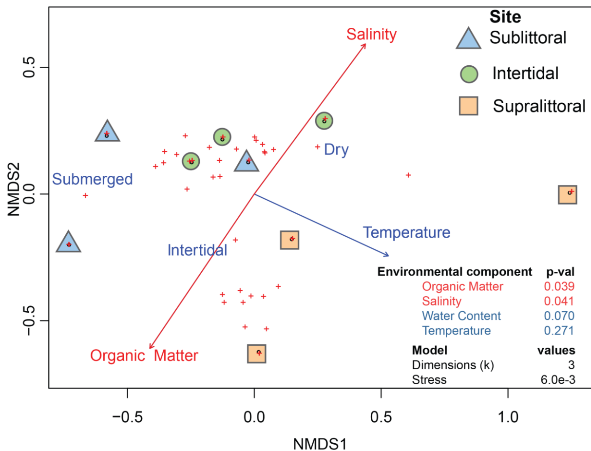
Fig. 3. Correlation between environmental variables and prokaryotic communities. Dots represent taxonomic abundances per site as plotted by Vegan metaMDS using nonmetric multidimensional scaling (NMDS). Arrow length is a representative of the predictor strength of environmental variable vectors, with red arrows having statistical significance as calculated by envfit (p-value \leq 0.05 ).
