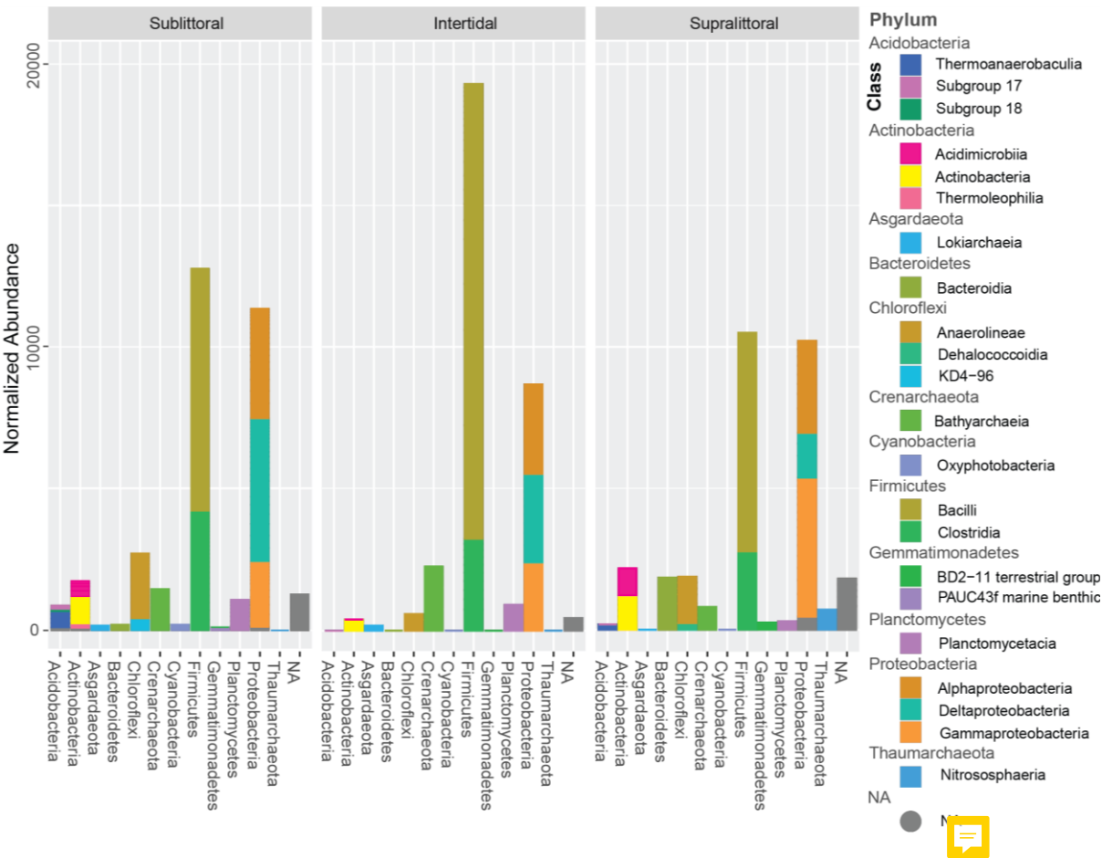
Fig 2. Normalized taxonomic abundances from each tidal zone. Taxa identified with abundance higher than 1% are shown as stacked bar plots, the horizontal axis is the Phylum level while the stacked bars are the Class level. Taxa abundance has been normalized by downsampling sequence depth.
