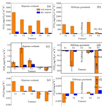
Fig. 6 Spatiotemporal patterns of CO 2 (first line), CH 4 (second line), and N 2 O (third line) emissions ( F ) in the upstream (T1, T2, and T3) and downstream areas (T4 and T5). Bars are the mean values for each transect and error bars are the standard errors.
