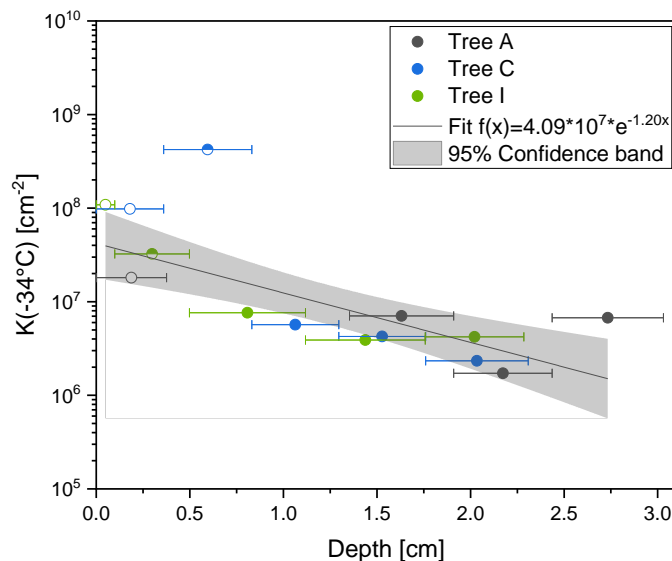
Figure 4: Cumulative nucleus concentration at -34\text{ }^{\circ}\text{C} ( K(-34^{\circ}\text{C}) ) of the analysed core samples of Tree A (grey), Tree C (blue) and Tree I (green). Bark samples are marked with a hollow symbol, bast samples are marked with a half-filled symbol. Filled symbols correspond to inner wood samples. To assign the depth of the different core segments, the centre of the segments was used. The sizes of the segments are visualized with corresponding horizontal lines. INM concentration increases towards outer layers of the trunk. The bast sample from Tree A does not freeze heterogeneously.
