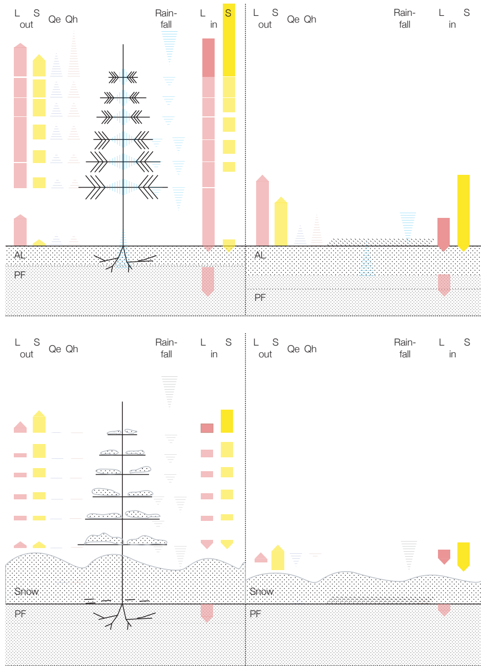
Figure 2. Schematic of the surface energy and water balance of the forest (left) and grassland (right) schemes for (a) snow-free period and (b) snow-covered period. The active layer (AL), the permafrost (PF), tree and grassland (dotted lines) and the snow-pack (Snow) in the snow covered period. In each of the four panels, incoming and outgoing longwave ( L_{in} , L_{out} ), incoming and outgoing solar ( S_{in} , S_{out} ), turbulent fluxes ( Q_h and Q_e ), the storage heat flux ( Q_s ), and precipitation (and interception) of rain- and snowfall are shown.
