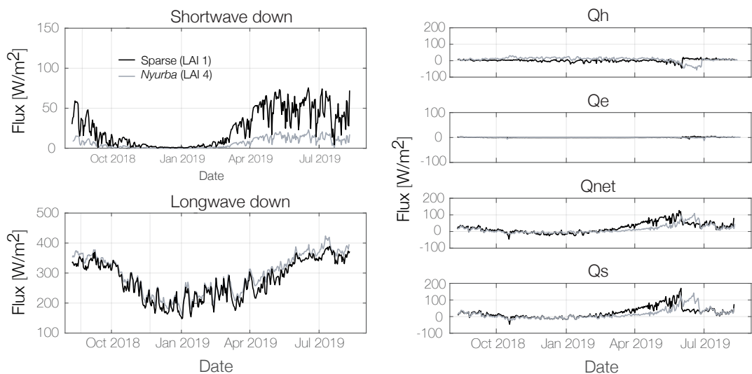
Figure 8. Left, modeled longwave and solar radiation at the forest ground for LAI = 1 m 2 m -2 (Sparse, black) and LAI = 4 m 2 m -2 (Nyurba, grey). Right, modeled turbulent fluxes ( Q_h and Q_e ), net radiation ( Q_{net} ) and storage heat flux at the forest ground ( Q_s ).
