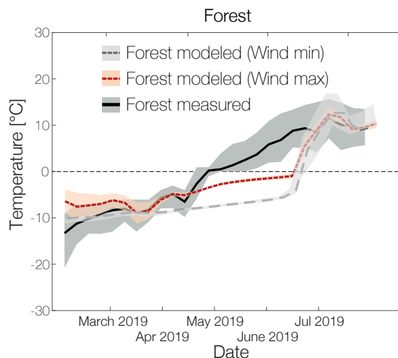
Figure 9. Modeled (Wind min (grey) and Wind max (red)) and measured (black) average weekly GST in 0.03 m depth in forest with standard deviation for modeled (light grey and light red) and measured (dark grey). Red represents a simulation using the wind speed at the top of the canopy as the input value for snow compaction. Grey shows the standard model simulation using the wind speed at the canopy bottom for the snow compaction mechanisms.
