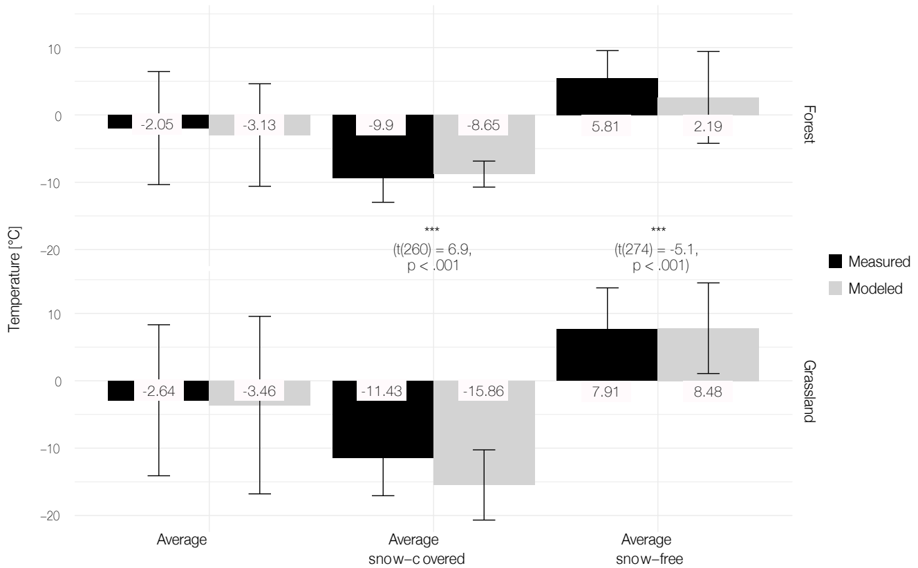
Figure 5. Average measured and modeled snow-covered period GST, average measured and modeled snow-free period GST, annual average measured and modeled GST and the respective standard deviations in forest (top, at 0.03 m depth) and grassland (bottom, at 0.07 m depth) over a measurement period of 1 year (10. August 2018 - 10. August 2019). The bars indicate mean values while the whiskers show the corresponding standard deviations. Unpaired t-test between modeled forest and grassland GST shows a statistically significant temperature difference for snow-covered and snow-free periods.
