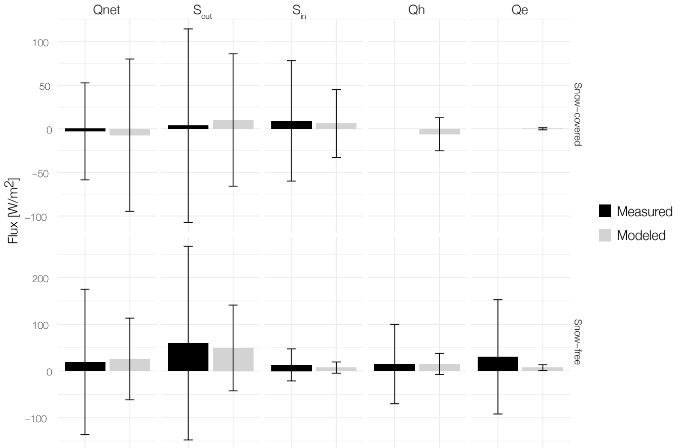
Figure C1. Modeled (grey) incoming and outgoing solar radiation ( S_{in} , S_{out} ) and turbulent fluxes ( Q_h , Q_e , Q_{net} ) for snow-covered (28.10.2017-27.04.2018, above) and snow-free (10.10.2017-27.10.2017 and 28.04.2018-10.10.2018, below) periods at the ground surface of forest. The bars indicate median values while the whiskers show the corresponding standard deviations.
