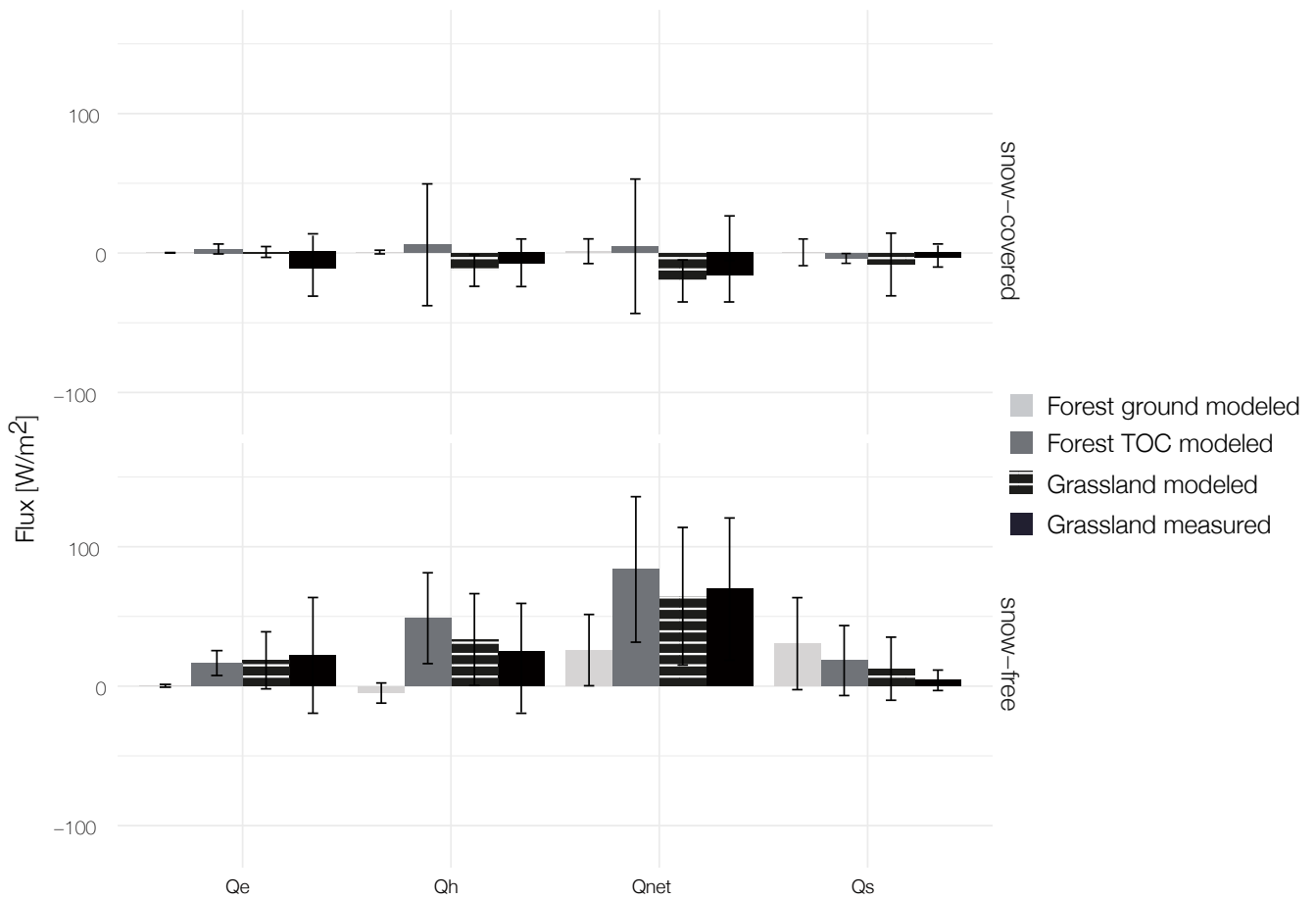
Figure 3. Surface energy balance for snow-covered (28.10.2018-27.04.2019) and snow-free (10.10.2019-27.10.2019 and 28.04.2019-10.10.2019) periods at the ground surface of grassland and forest and at the top of the canopy of forest (Forest TOC). Shown are the net radiation ( Q_{net} ), sensible ( Q_h ), latent ( Q_e ) and storage heat flux ( Q_s ) for the model runs of the forest and grassland site as well as the measured values at the grassland site. The bars indicate mean values while the whiskers show the corresponding standard deviations.
