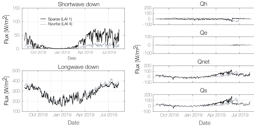
Figure 8. Left, modeled longwave and solar radiation at the forest ground for \text{LAI} = 1 \text{ m}^2 \text{ m}^{-2} (Sparse, black) and \text{LAI} = 4 \text{ m}^2 \text{ m}^{-2} (Nyurba, grey). Right, modeled turbulent fluxes ( Q_h and Q_e ), net radiation ( Q_{net} ) and storage heat flux at the forest ground ( Q_s ).
