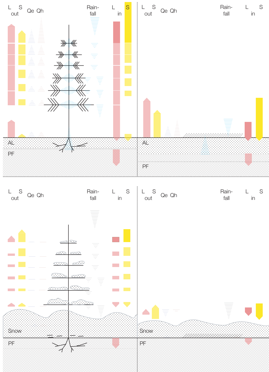
Figure 2. Schematic of the surface energy and water balance of the forest (left) and grassland (right) schemes for top, the snow-free period and bottom, the snow-covered period. The active layer (AL), the permafrost (PF), tree and grassland (dotted lines) and the snow-pack (Snow) in the snow covered period. In each of the four panels, incoming and outgoing longwave ( L_{in} , L_{out} ), incoming and outgoing solar ( S_{in} , S_{out} ), turbulent fluxes ( Q_h and Q_e ), the storage heat flux ( Q_s ), and precipitation (and interception) of rain- and snowfall are shown.
