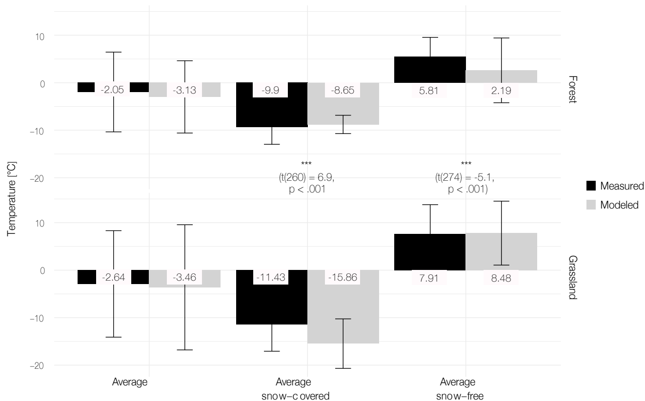
Figure 5. Average measured and modeled snow-covered period GST, average measured and modeled snow-free period GST, annual average measured and modeled GST and the respective standard deviations in forest (top, at 0.03 m depth) and grassland (bottom, at 0.07 m depth) over a measurement period of 1 year (10. August 2018 - 10. August 2019). The bars indicate mean values while the whiskers show the corresponding standard deviations. Unpaired t-test between modeled forest and grassland GST shows a statistically significant temperature difference for snow-covered and snow-free periods.
