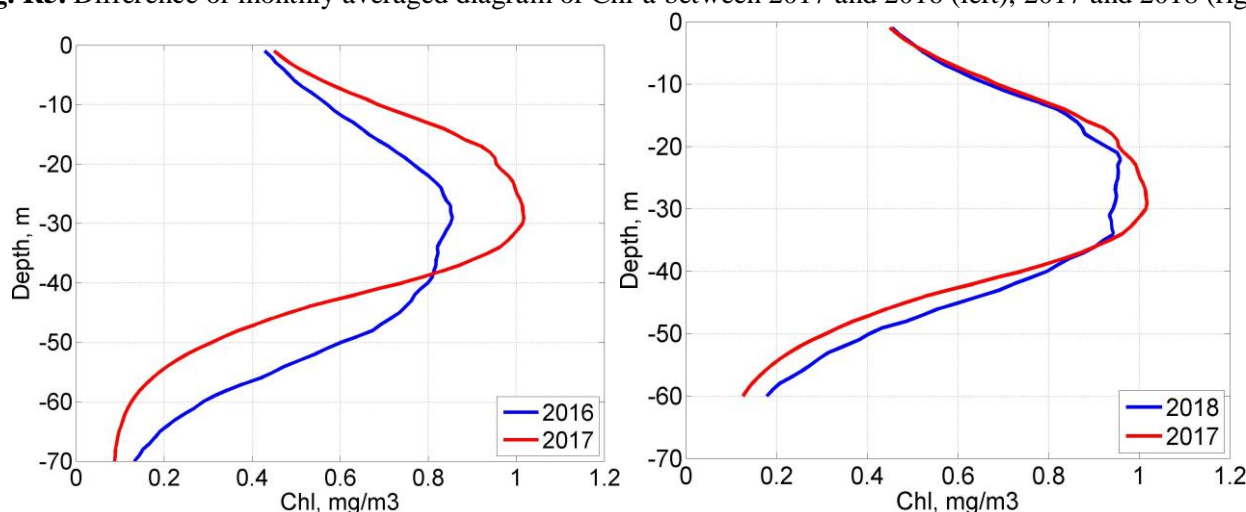
Fig. R6. Average profile of Chl in 2016 and 2017 (left), 2017 and 2018 (right) by Bio-Argo buoy measurements (right).
