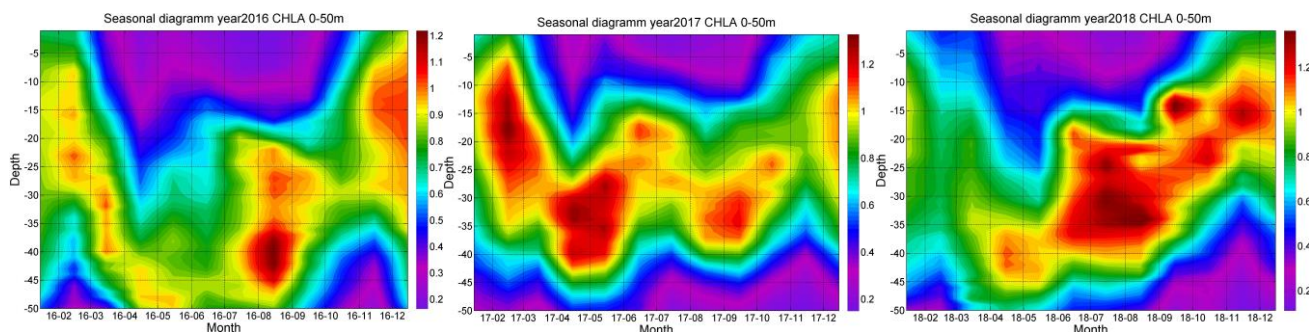
Fig. R4. Seasonal diagrams of Chl-a in 2016, 2017, and 2018 years from Bio-Argo data.
