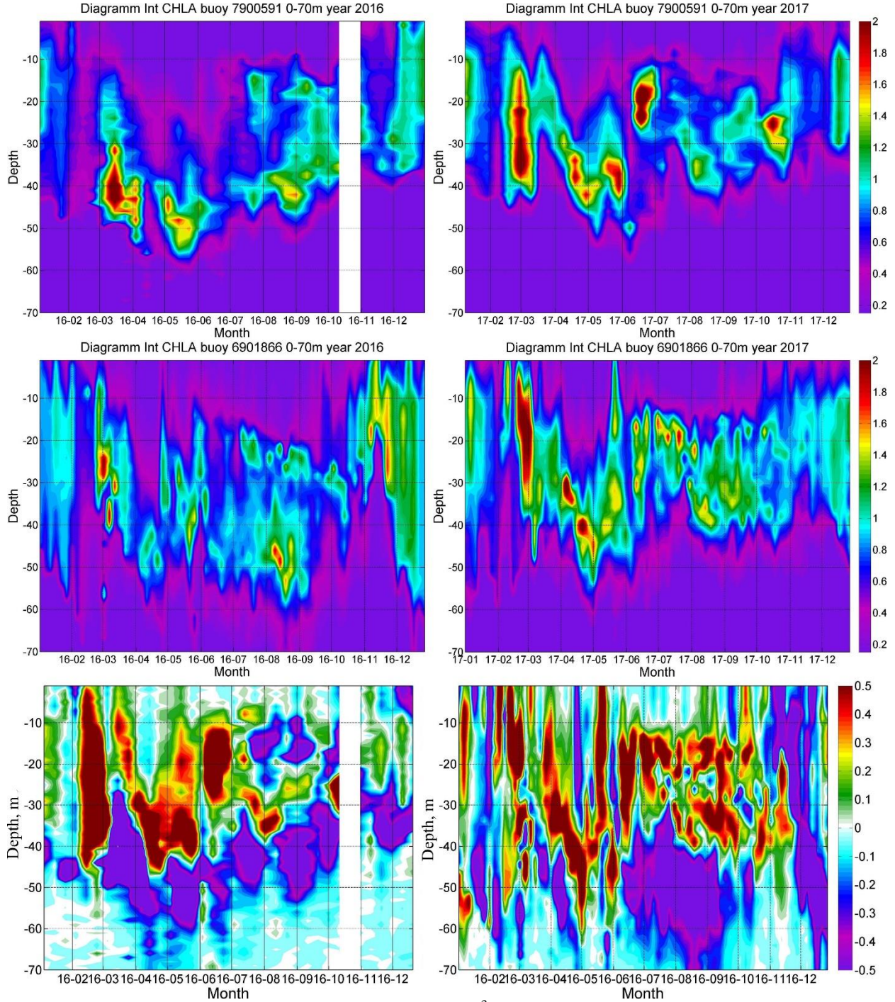
Fig. R2. Time variability (5-days averaging) of Chl-a ( \text{mg}/\text{m}^3 ) by the measurements of Bio-Argo buoy #7900591 (top panel) and buoy #6901866 (central panel) in 2016 (left) and 2017 (right). Bottom panel – the differences between 2017 and 2016 by buoy #6901866 (left) and buoy #7900591 (right).
