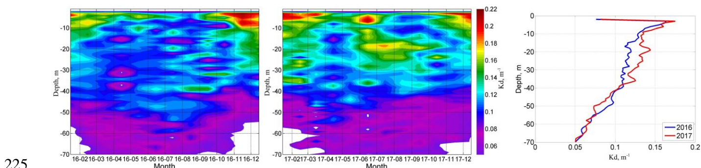
225 Fig. R7. Monthly-averaged vertical distribution of K_d (PAR) in 2016 (left) and 2017 (center), K_d yearly-averaged profile in 2016 and 2017 (right) in the Black Sea from Bio-Argo data.
