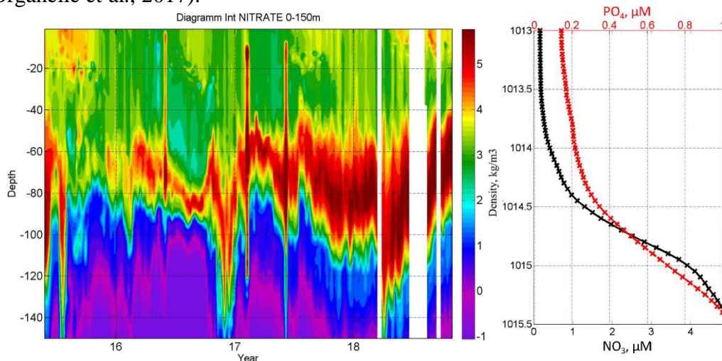
Fig. R1: left – Interannual diagram of NO 3 ( \mu\text{M} ) measured by buoy Bio-Argo; right – multiannual averaged vertical profiles of NO 3 ( \mu\text{M} , black line) and PO 4 ( \mu\text{M} , red line) for October shown in \sigma -coordinates.
