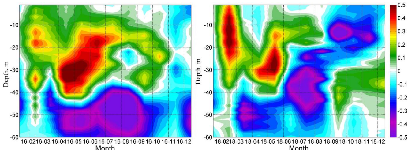
Fig. R5. Difference of monthly averaged diagram of Chl-a between 2017 and 2016 (left), 2017 and 2018 (right).
