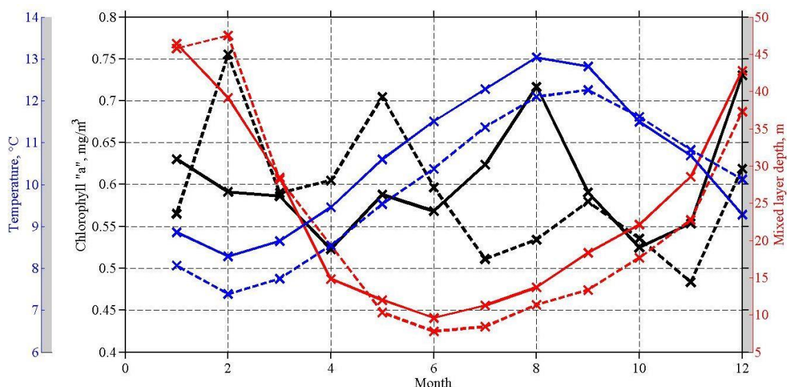
Fig. R8. Average seasonal variability of Chl, temperature and mixed layer depth in 2016 (solid line) and 2017 (dashed) in the 0-70 m layer.
