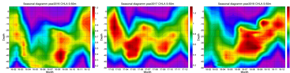
Fig. 4. Fig. R4. Seasonal diagrams of Chl-a in 2016, 2017, and 2018 years from Bio-Argo data.
