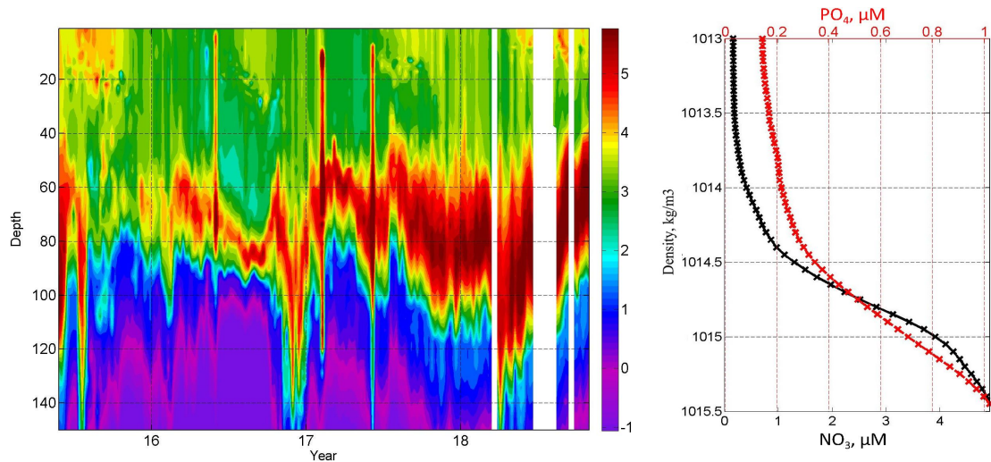
Fig. 1. Fig. R1: left– Interannual diagram of \text{NO}_3 ( \mu\text{M} ) measured by buoy Bio-Argo; right– multiannual averaged vertical profiles of \text{NO}_3 ( \mu\text{M} , black line) and \text{PO}_4 ( \mu\text{M} , red line) for October shown in \sigma -coordinate
