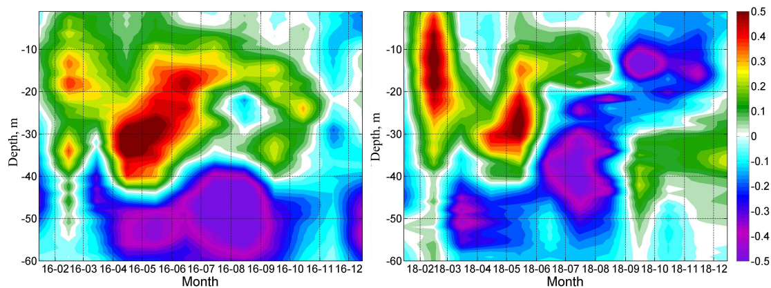
Fig. 5. Fig. R5. Difference of monthly averaged diagram of Chl-a between 2017 and 2016 (left), 2017 and 2018 (right).
