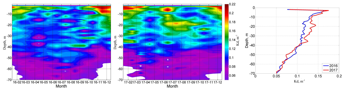
Fig. 7. Fig. R7. Monthly-averaged vertical distribution of K_d (PAR) in 2016 (left) and 2017 (center), K_d yearly-averaged profile in 2016 and 2017 (right) in the Black Sea from Bio-Argo data.
