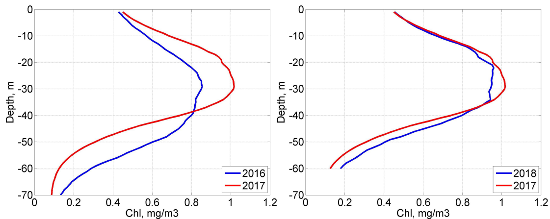
Fig. 6. Fig. R6. Average profile of Chl in 2016 and 2017 (left), 2017 and 2018 (right) by Bio-Argo buoy measurements (right).
