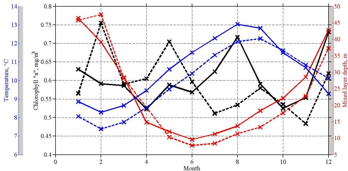
Fig. 8. Fig. R8. Average seasonal variability of Chl, temperature and mixed layer depth in 2016 (solid line) and 2017 (dashed) in the 0-70 m layer.
