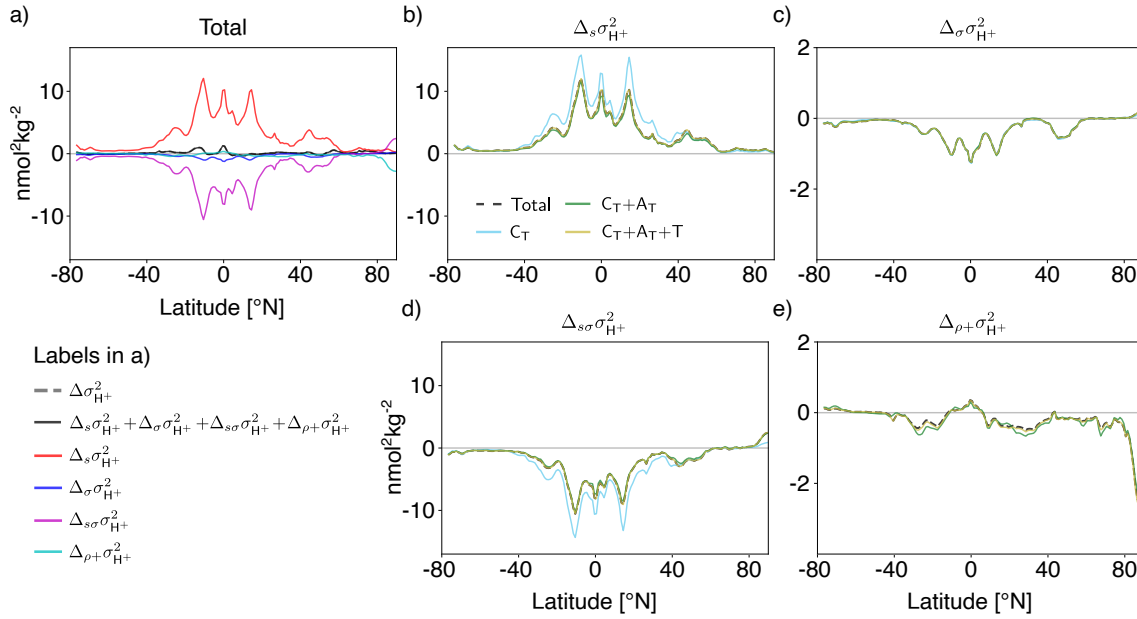
Figure 10. Decomposition of [H^+] variability changes at 200 m into different drivers ( C_T , A_T , temperature, and salinity). Shown are changes from preindustrial to 2081-2100 following the RCP8.5 scenario. The simulated change in [H^+] variance ( \Delta\sigma_{H^+}^2 ) is decomposed into the contribution from changes in the sensitivities that arise from changes in the drivers' mean values ( \Delta_s\sigma_{H^+}^2 ), the contribution from changes in the drivers' standard deviations ( \Delta_\sigma\sigma_{H^+}^2 ), the contribution from simultaneous changes in the sensitivities and the drivers' standard deviations ( \Delta_{s\sigma}\sigma_{H^+}^2 ), and the contribution from correlation changes alone together with simultaneous changes in correlations and sensitivities and standard deviations ( \Delta_\rho\sigma_{H^+}^2 ) (a). The contributions to these components from changes in C_T alone (light blue lines), from changes in C_T and A_T (green lines), and from C_T , A_T and temperature (gold lines) are shown in panels (b-e). The dashed black lines in panels (b-e) show the total components that contain contributions from all four drivers.
