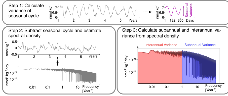
Figure 2. The three-step decomposition of [H^+] variance into interannual, seasonal, and subannual variance, exemplified for a surface grid cell at 40° N and 30° W in the North Atlantic at preindustrial. In a first step, the climatological seasonal cycle is determined (over the whole period, only five years are depicted here) and its variance is calculated. Note that the seasonal cycle in this grid cell has two minima and maxima. In a second step, the spectral density of the anomalies with respect to the seasonal cycle is calculated. In a third step, interannual and subannual variance is estimated from the spectral density.
