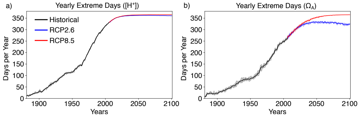
Figure 4. Simulated globally averaged yearly extreme days defined with respect to a fixed baseline for [H^+] using the preindustrial 99 th percentile (a) and for \Omega_A using the preindustrial 1 st percentile (b). Shown are changes at the surface over the 1881-2100 period following historical (black lines) and future scenarios, RCP8.5 (red) and RCP2.6 (blue). The thick lines display the five-member ensemble means and the shaded areas represent the maximum and minimum ranges of the individual ensemble members.
