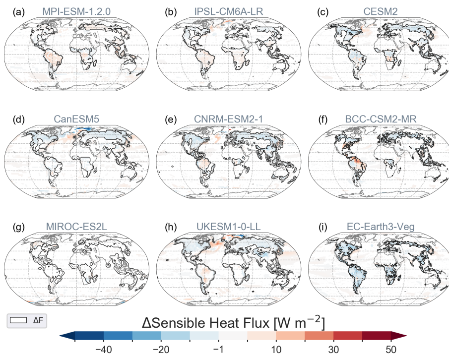
Fig. 3. Sensible heat fluxes
