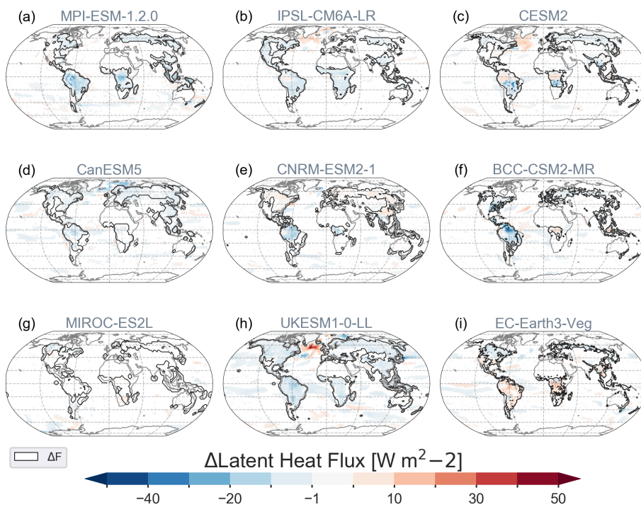
Fig. 2. Latent heat fluxes
