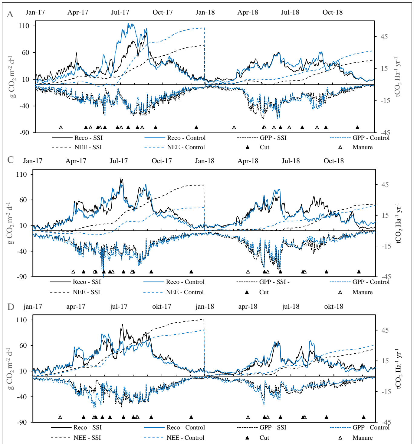
Figure B1 Daily Reco and GPP for location in g CO 2 m -2 d -1 on the primary y-axis, for control and SSI for locations A,C and D. Accumulative NEE in tCO 2 Ha -1 yr -1 , for control and SSI, every year starting at 0.
