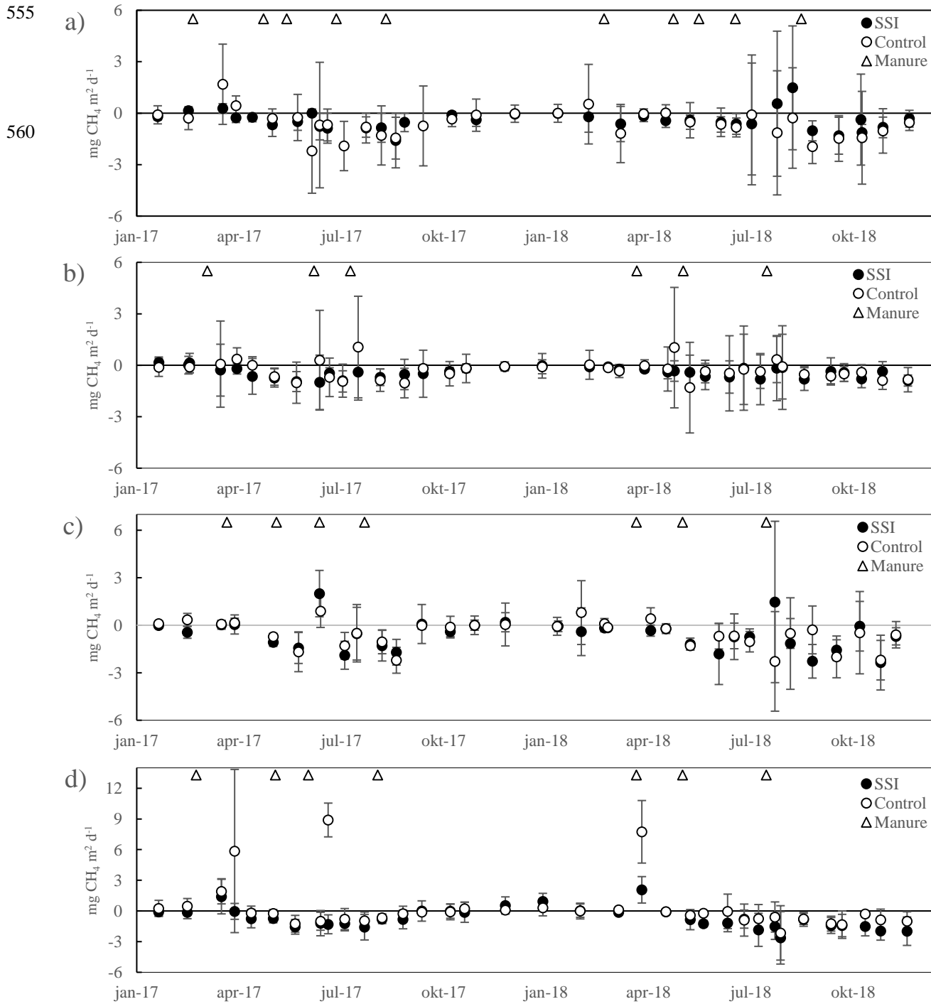
Figure C1 CH 4 exchange throughout 2017 and 2018 in mg CH 4 m -2 d -1
