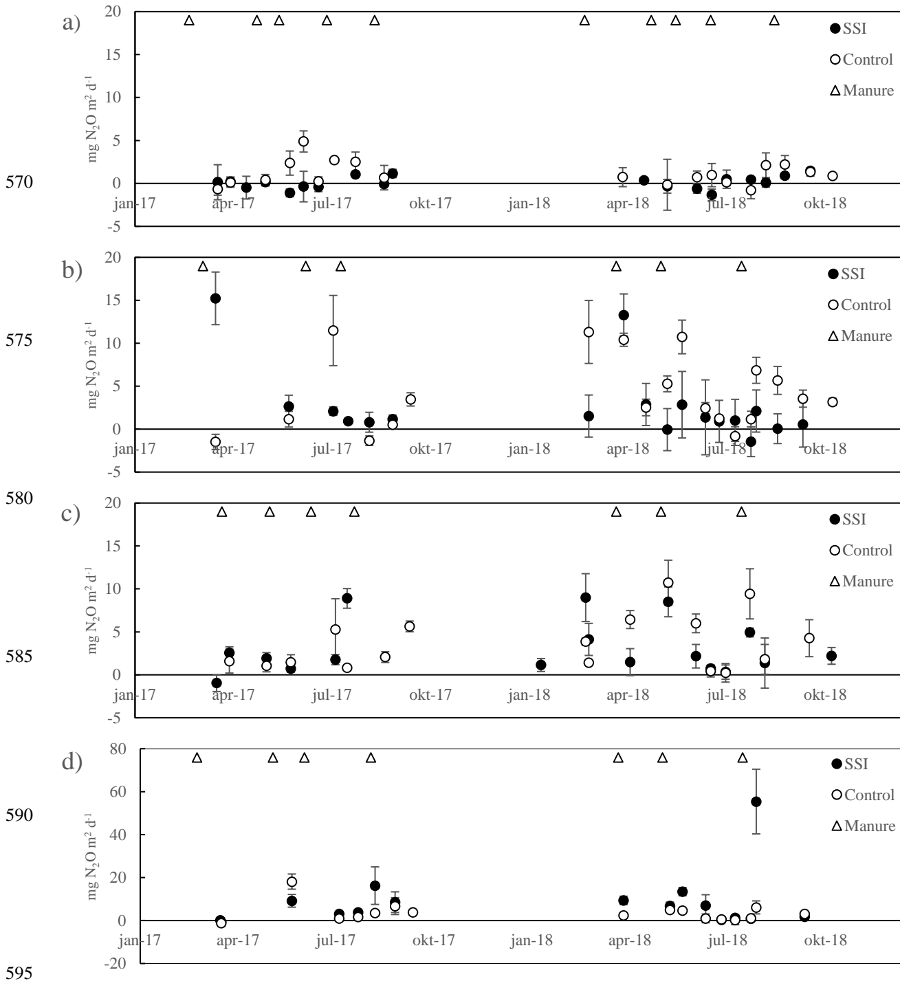
Figure D1 N 2 O exchange throughout 2017 and 2018 in mg N 2 O m -2 d -1 .
