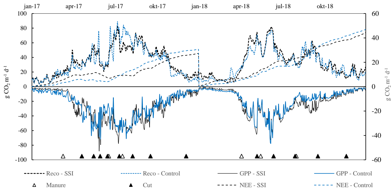
390 Figure 7 R_{\text{eco}} and GPP for location B in g CO 2 m -2 d -1 on the primary y-axis, for control and SSI. Accumulative NEE in t CO 2 ha -1 yr -1 , for control and subsoil irrigation (SSI), every year starting at 0.
