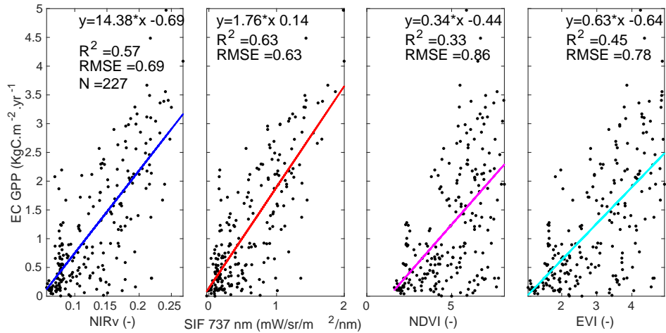
Figure 1. The relationship of NIRv, SIF, NDVI, and EVI with tower GPP. all correlations have a p-value < 10 -6 .
